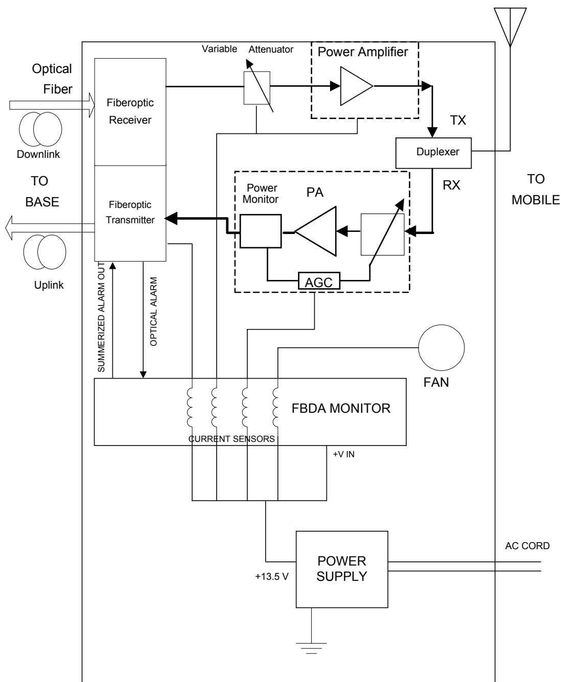
FBDA-PCS-AC-10W ELELCTRIC SCHEMATICS
