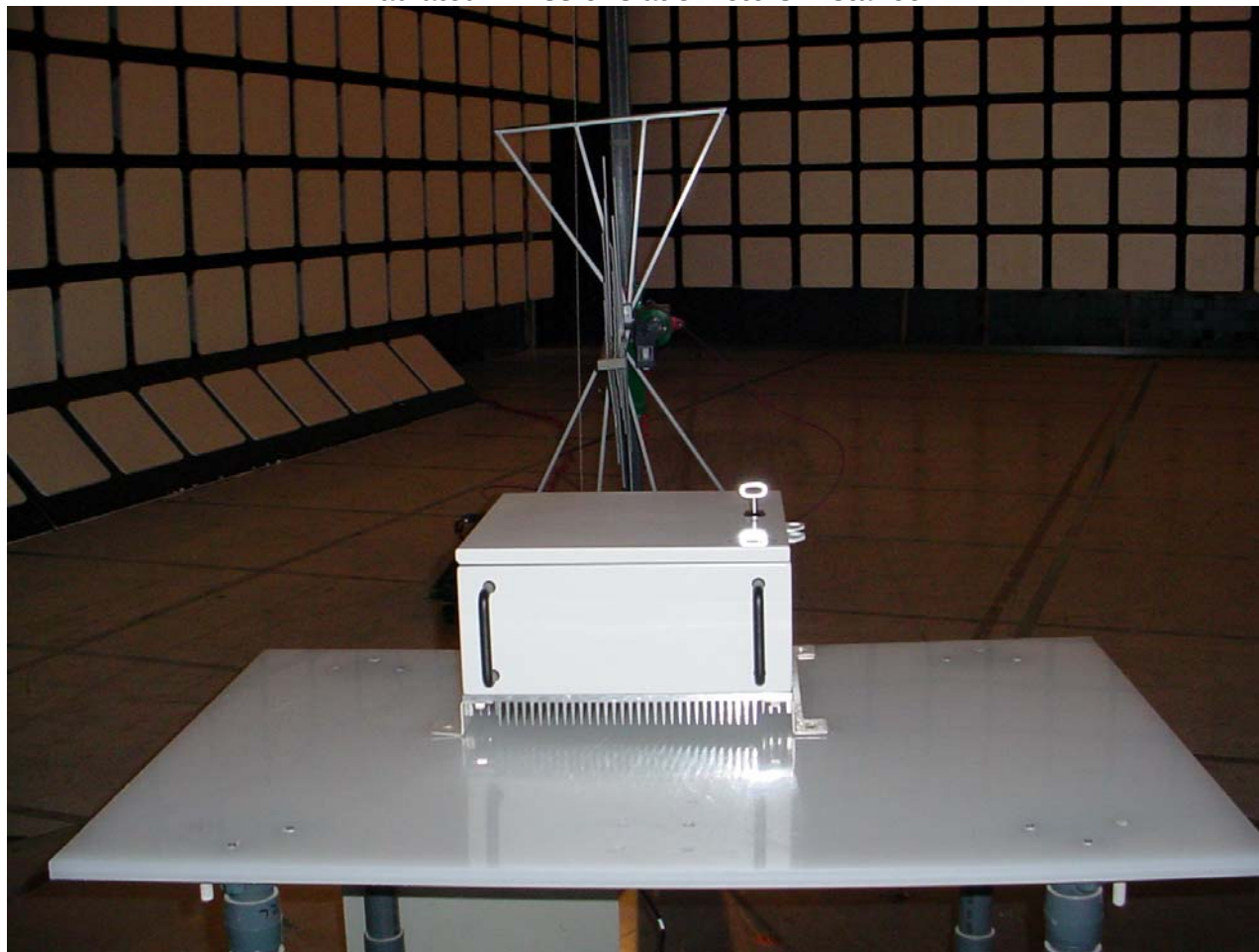
Radiated Emissions at 3 Meters Distance
