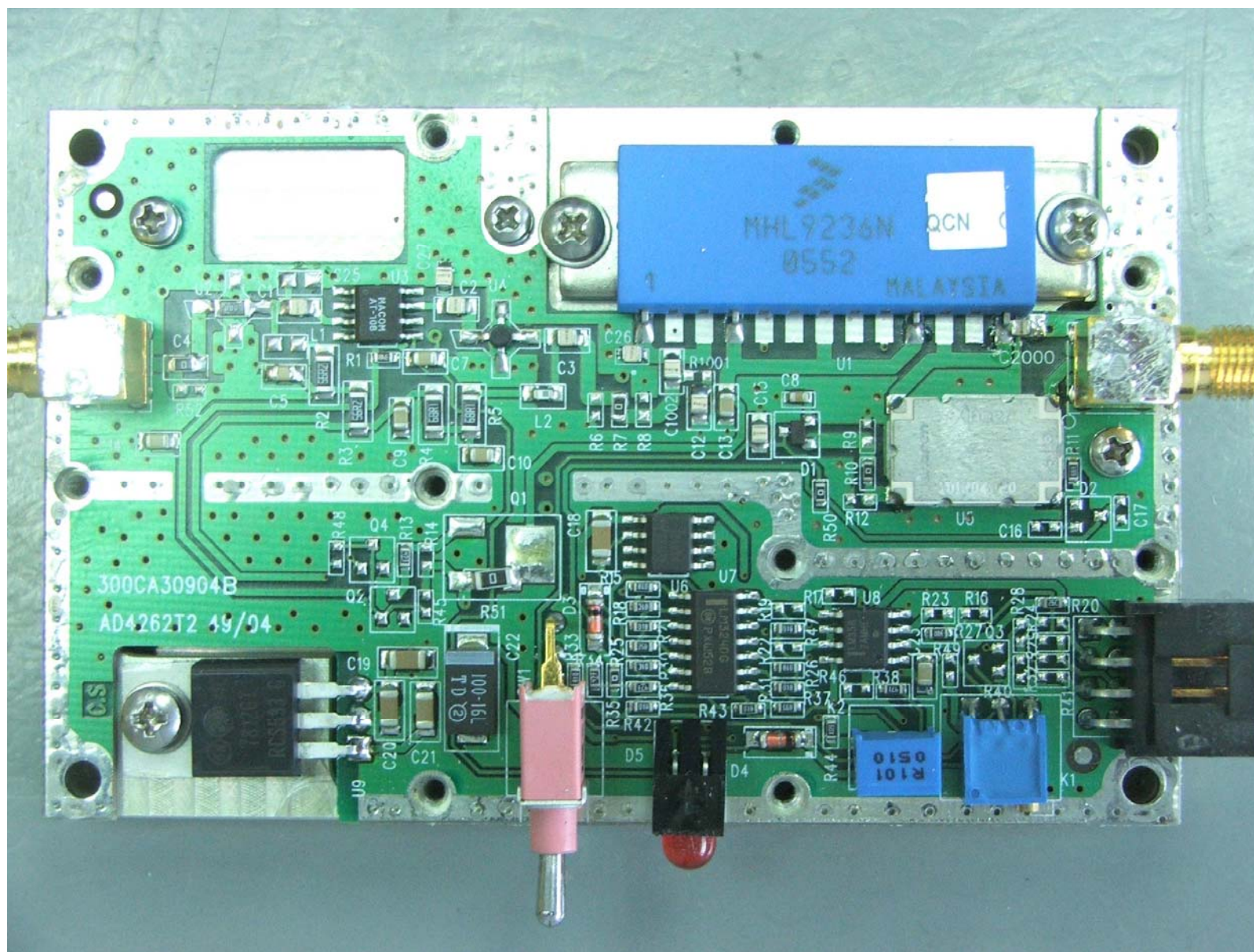
Dekolink Wireless Ltd. Dual Band Bi-Directional Amplifier, Model MW-CBDA-SMR-700-800-16W80 FCC ID: OIWBDASMR16W80
