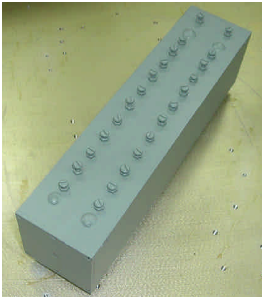
Photograph No.8 MW-BDA-ESMR-50W90 high power repeater Base diplexer first side view
