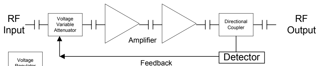
DOWN LINK POWER AMPLIFIER BLOCK DAIGRAM
