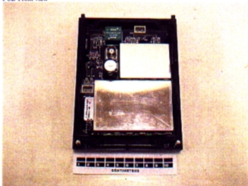
PCB-Front view
