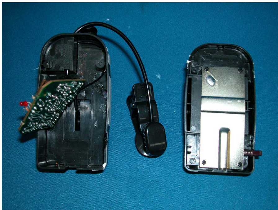
Assembly (View 2)
