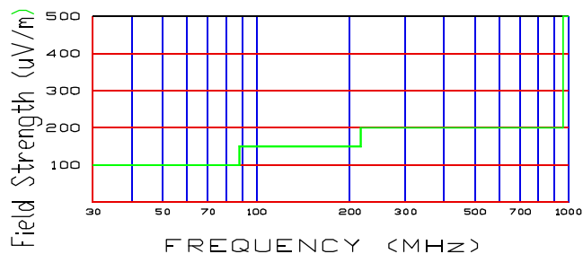
Fig. 14. Spurious Limits at 3 meters
