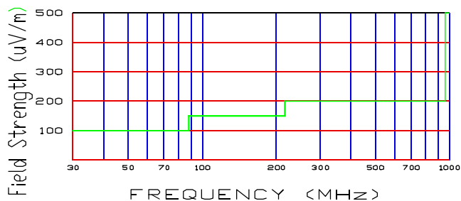
Fig. 12. Harmonic Limits at 3 meters
