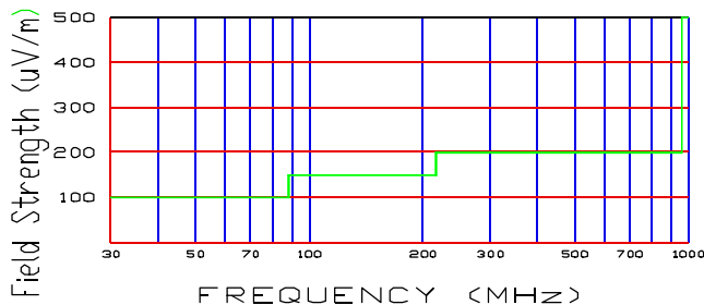
Fig. 11. Harmonic Limits at 3 meters
