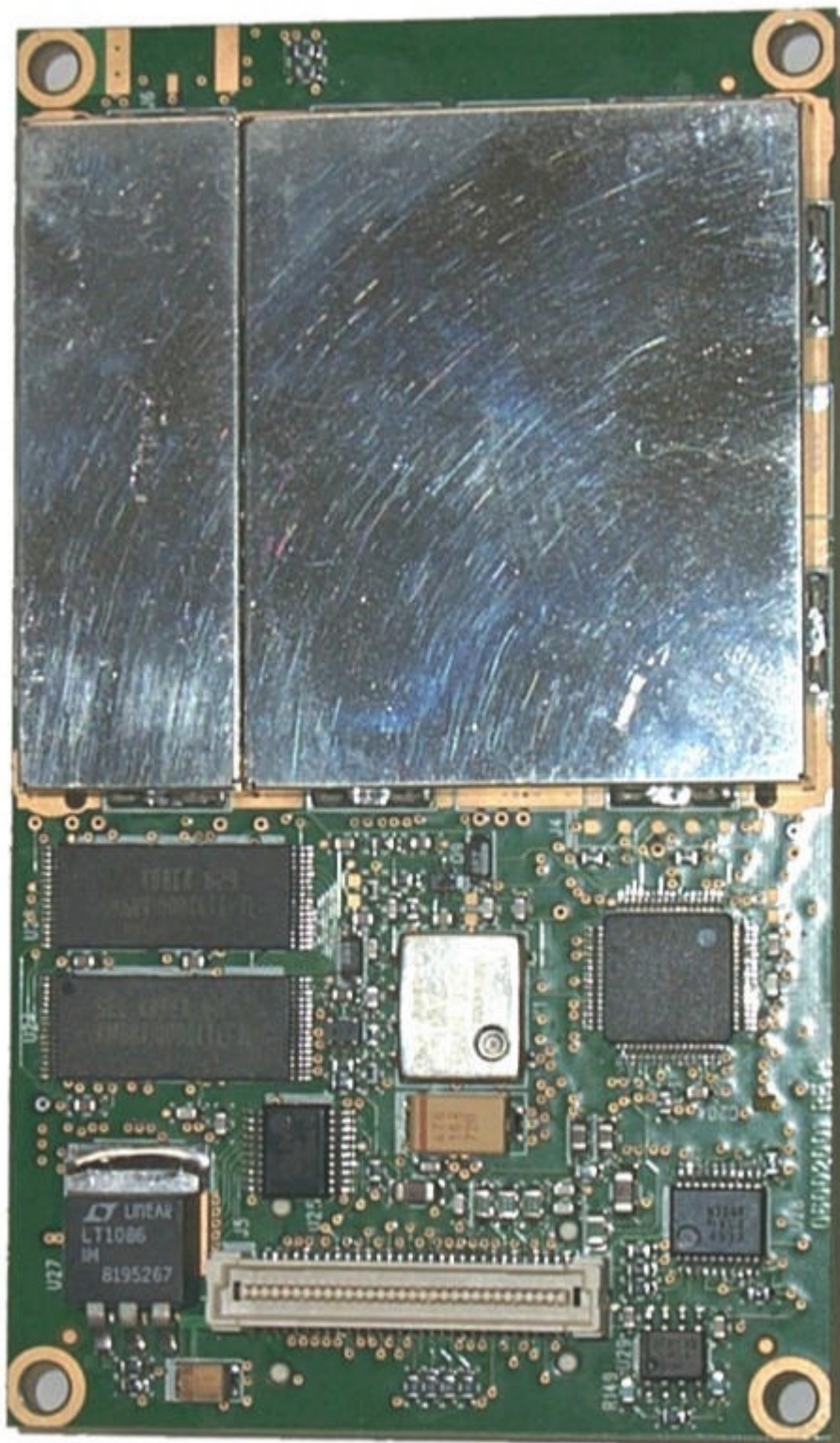
Photo 4. Bottom of RM PCB with RF shields covering radio circuitry.
