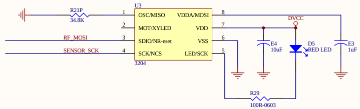
Optical Mouse Sensor
