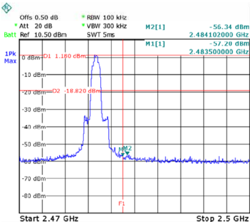
TX in 8DPSK Band edge-right side
