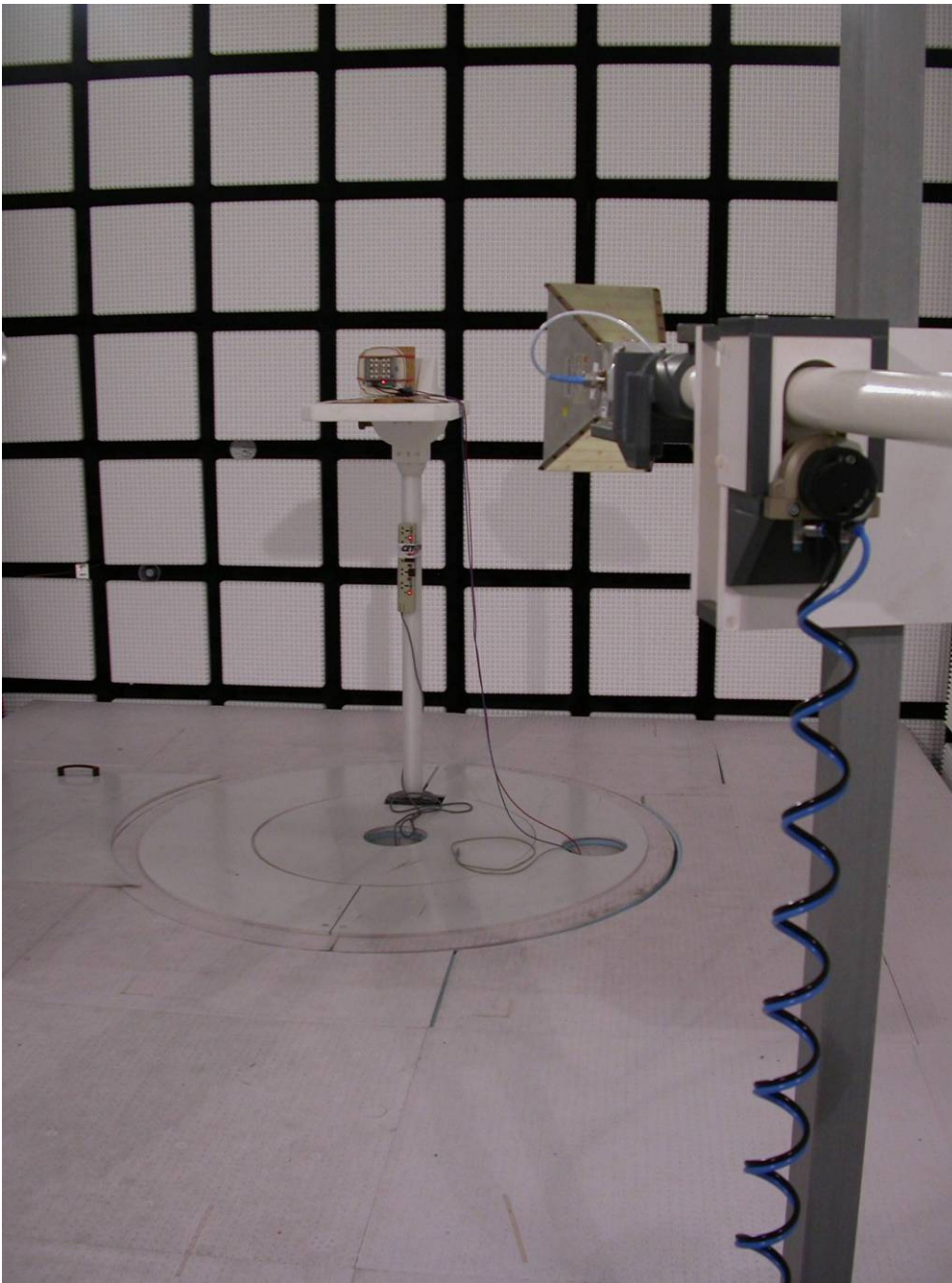
Spurious Emission measurement 1 GHz – 12 GHz
