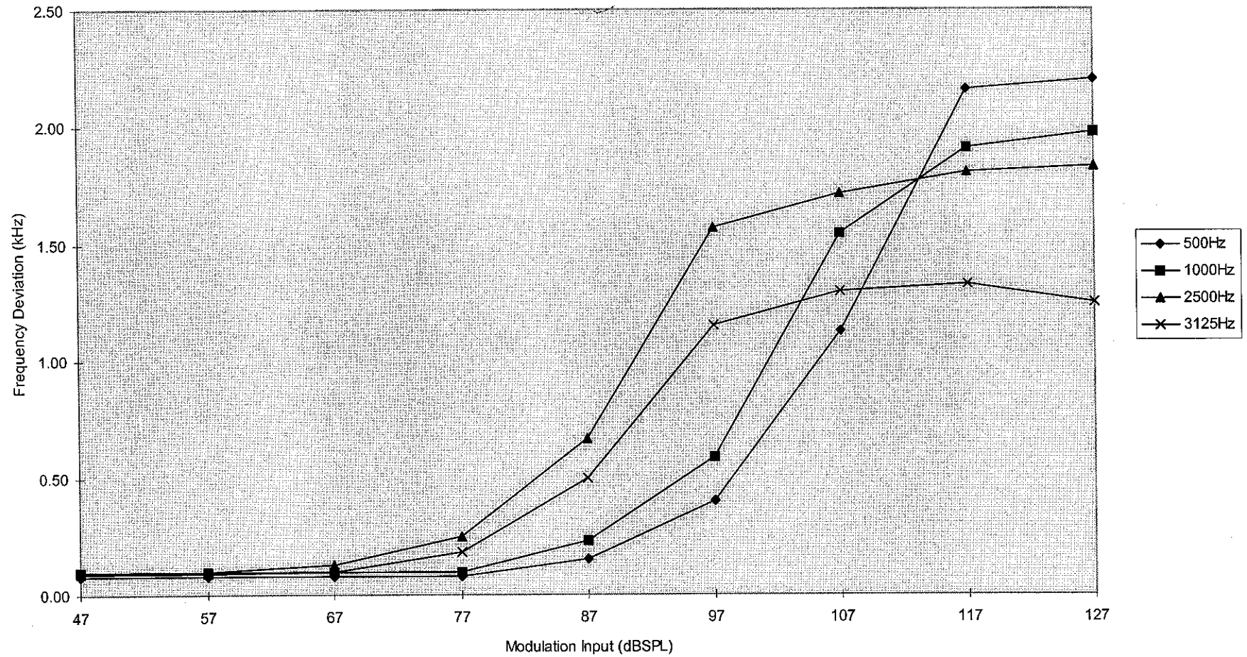
Modulation Limiting Characteristic
