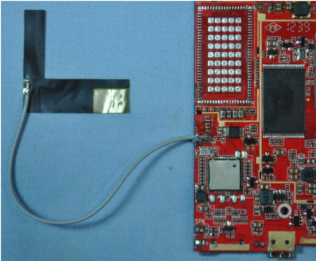
WiFi & BT module + Antenna
