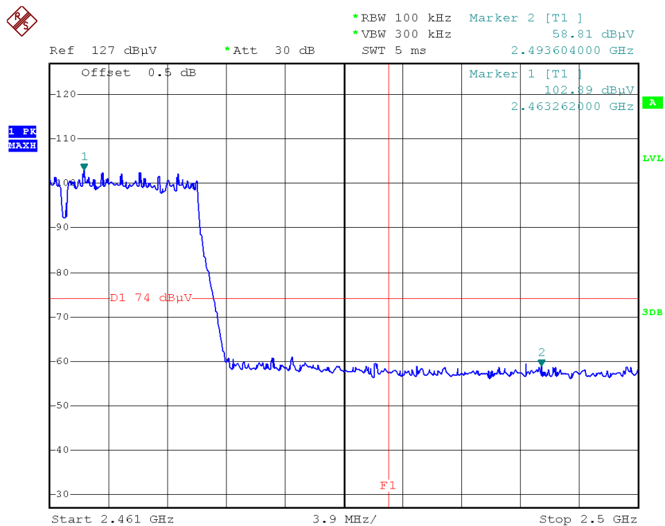
(Plot 2.5.1 C3: Channel = 11 Peak @ 802.11n-20)
