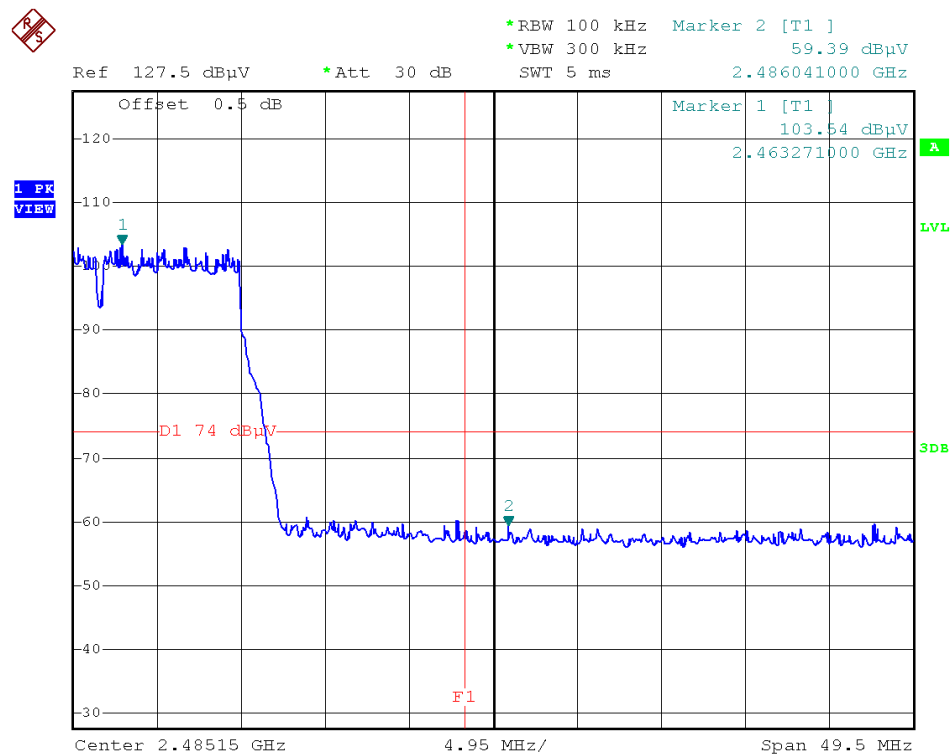
(Plot 2.5.1 B3: Channel = 11 Peak @ 802.11g)
