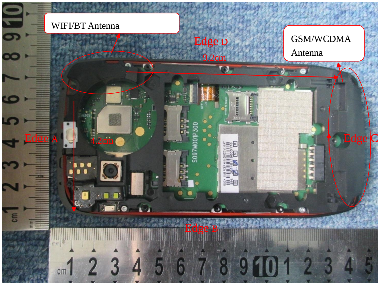
Fig. 3 Position of the antennas
