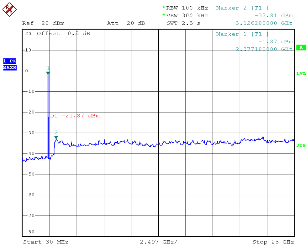
(Plot D.1: Channel = 0, 30MHz to 25GHz @ \pi/4 -DQPSK)
