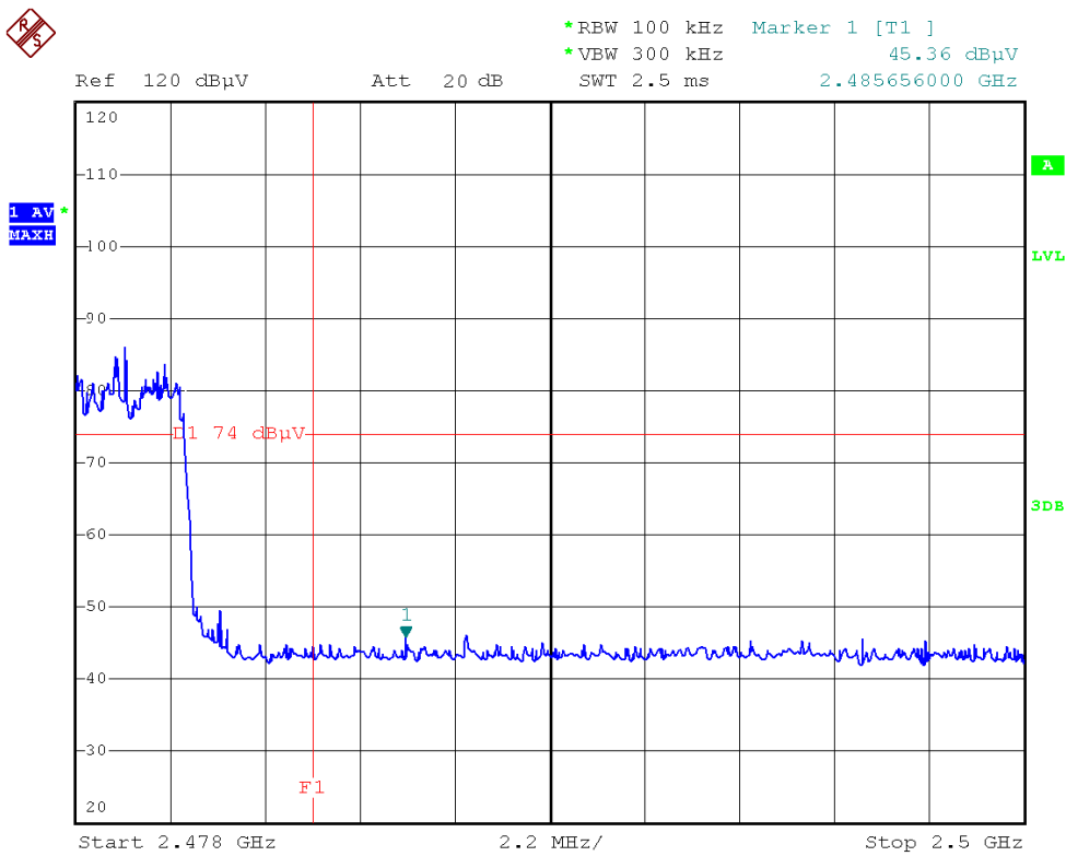
(Plot F2-1: Channel = 78 AVERAGE)
