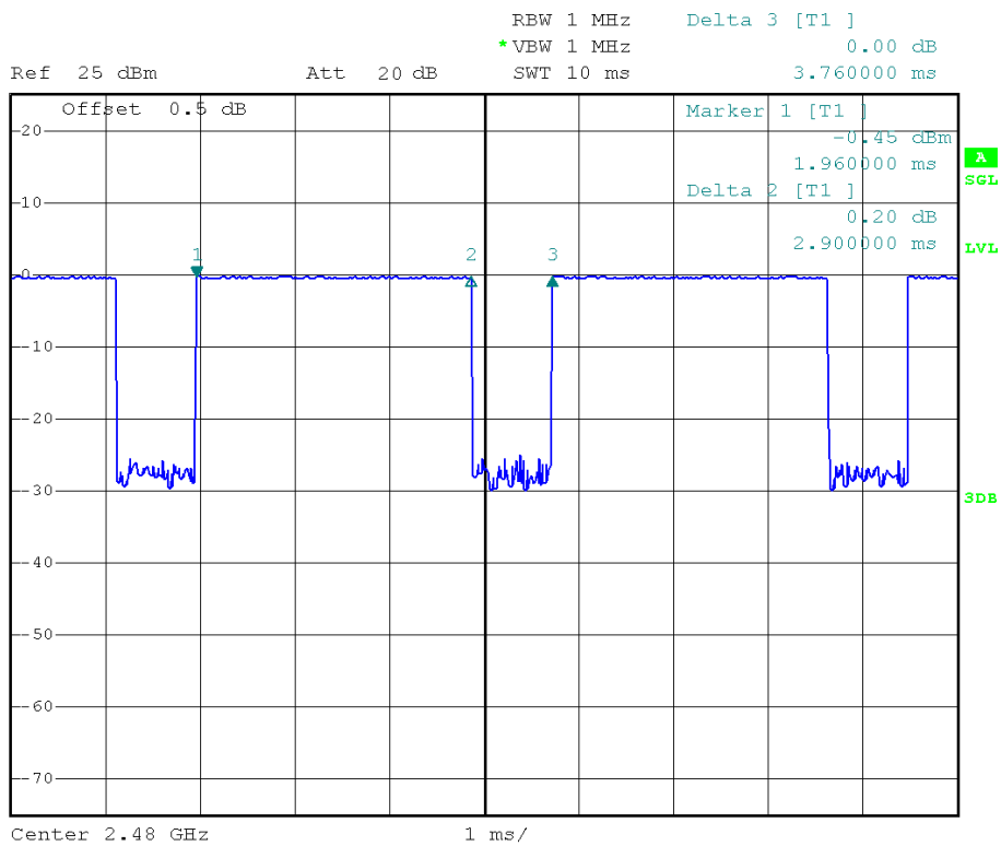
(Plot C: Channel = 2480 @ GFSK)
