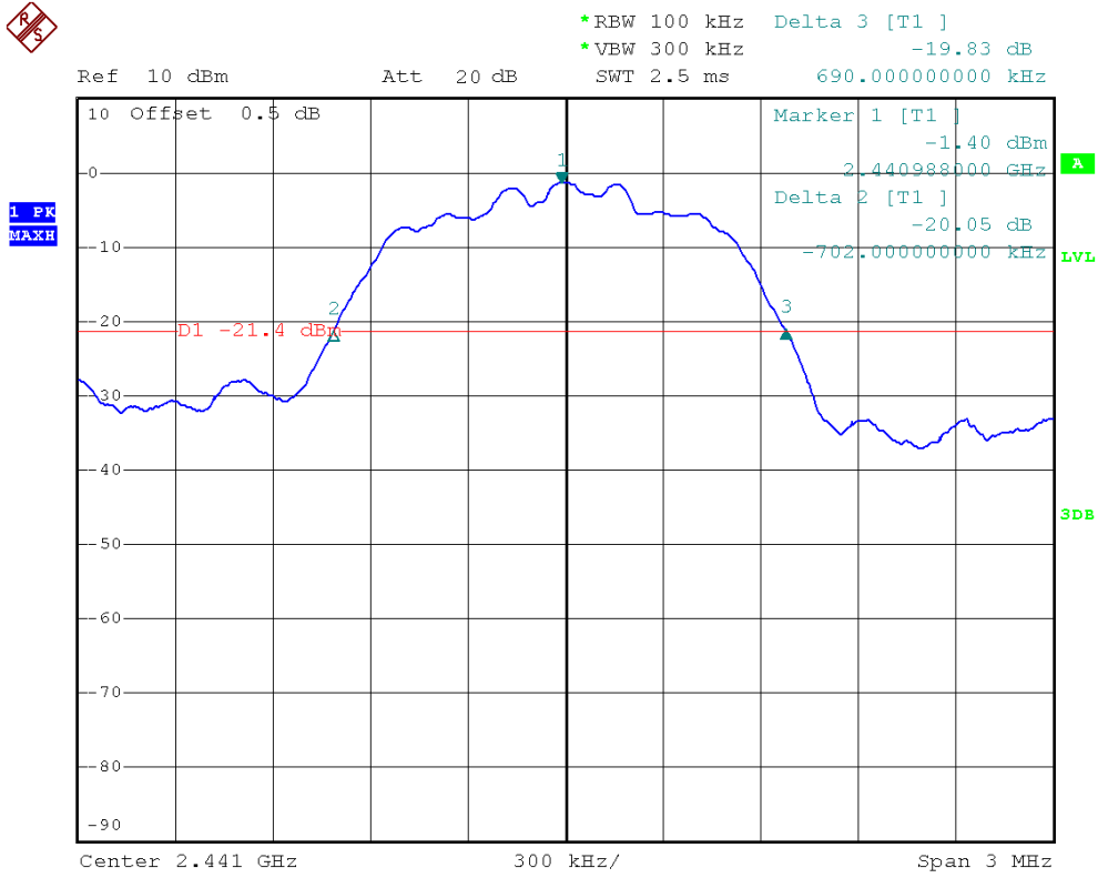
(Plot E: Channel = 2441 @ 1/4-DQPSK)
