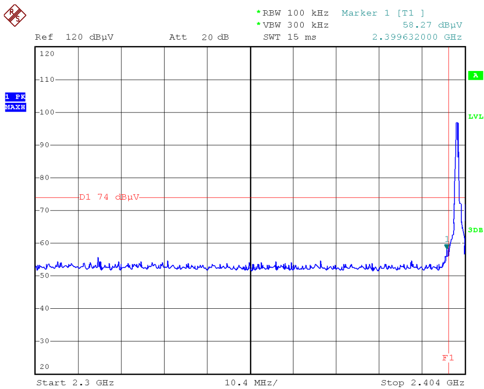
(Plot A1: Channel = 0 PEAK @ GFSK)
