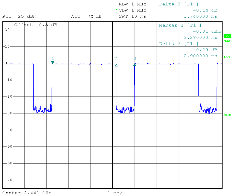
(Plot B: Channel = 2441 @ GFSK)
