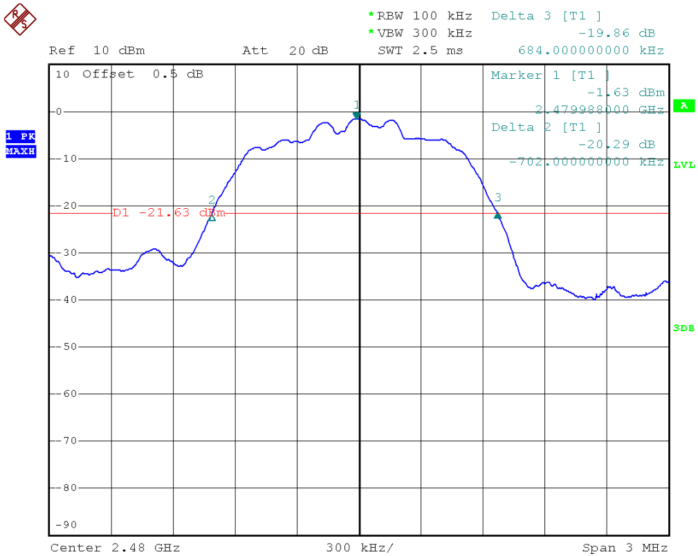
(Plot F: Channel = 2480 @ 1/4-DQPSK)
