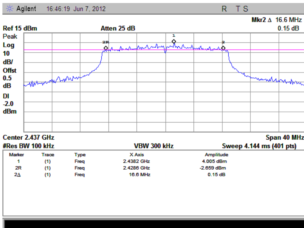
(Plot H: Channel 6: 2437MHz @ 802.11n)
