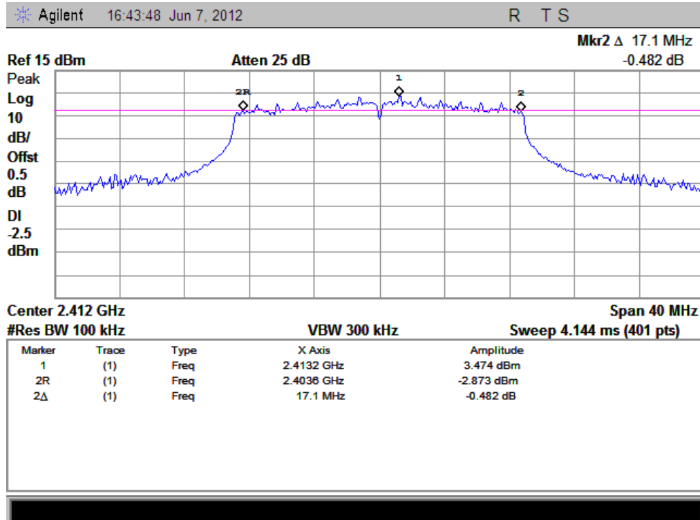
(Plot G: Channel 1: 2412MHz @ 802.11n)
