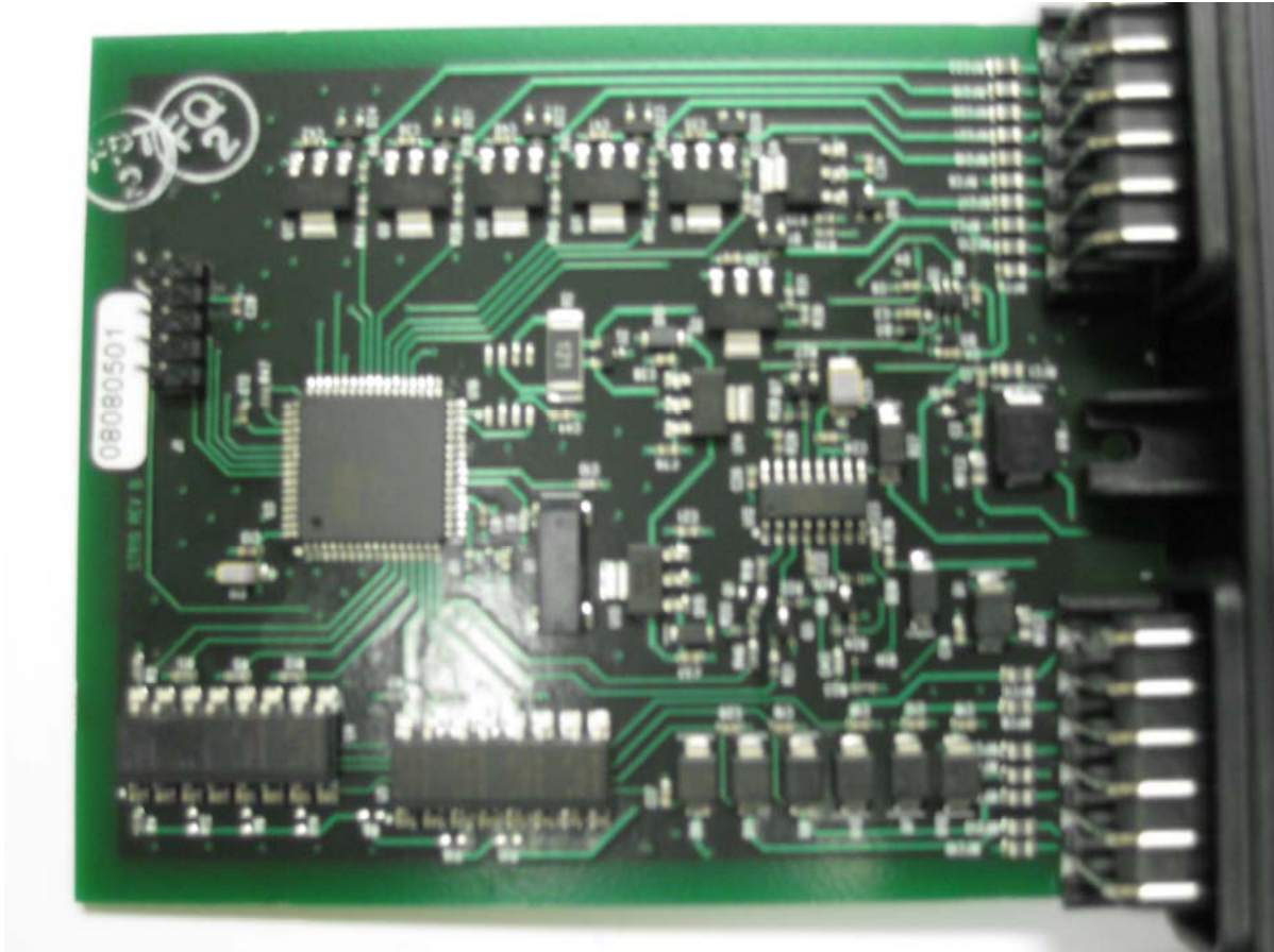
View #2 – Close up of RF Section
