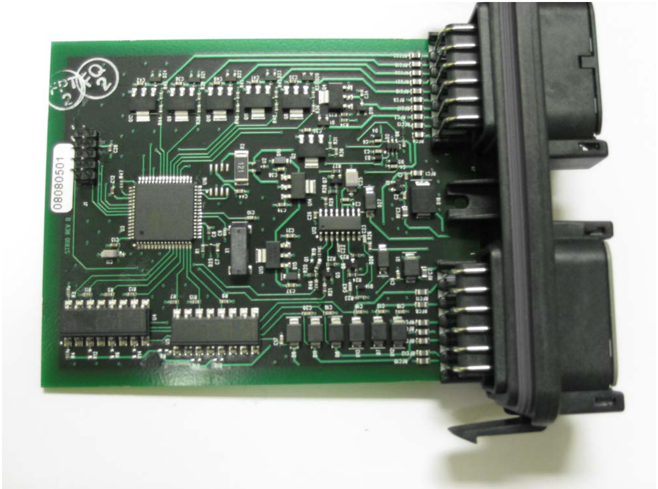
View #1 Close Up of RF Section
