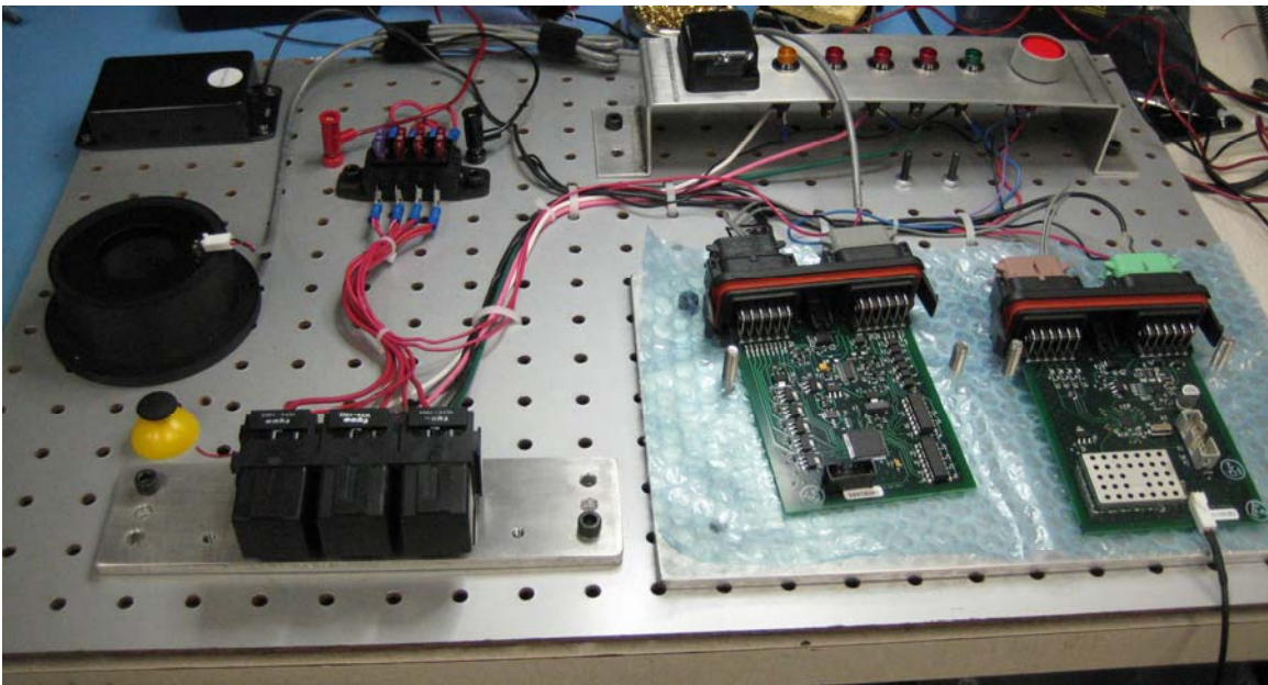
Test Setup
