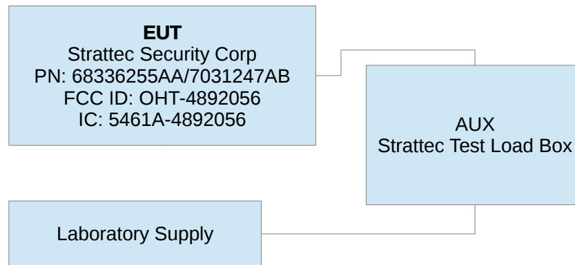
Figure 2: EUT Test Configuration Diagram.
