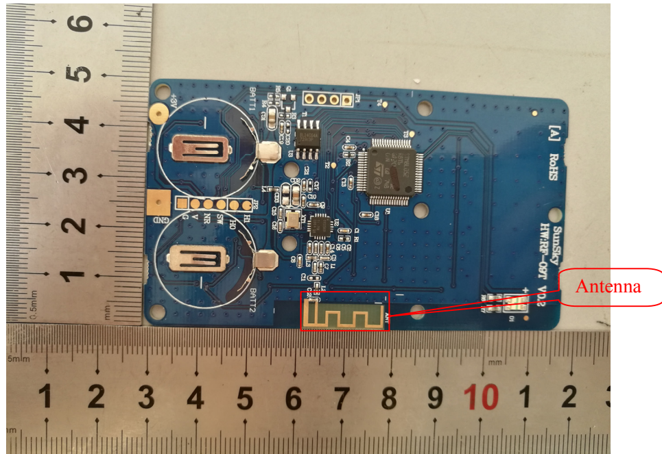
EUT – PCB Chip View
