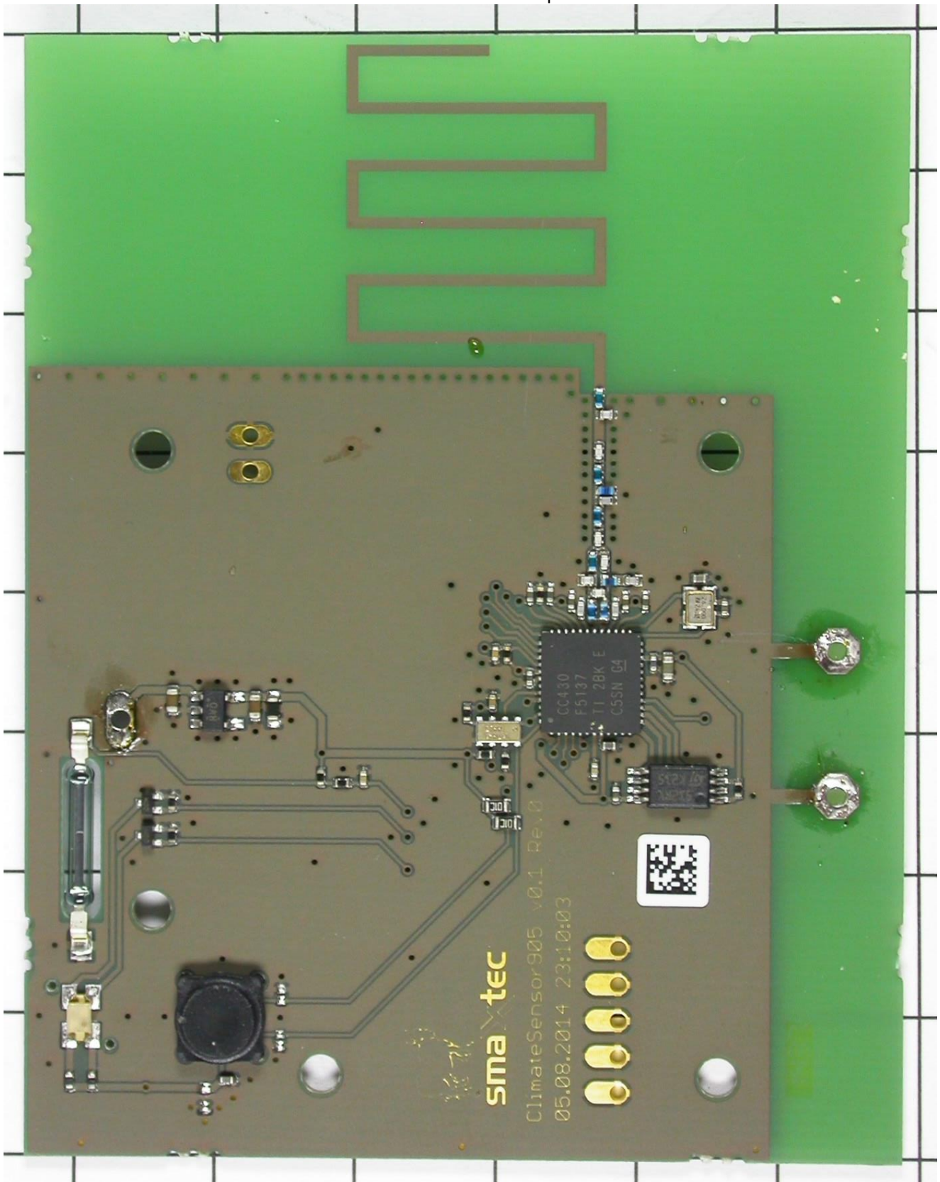
Climate sensor PCB – top view
