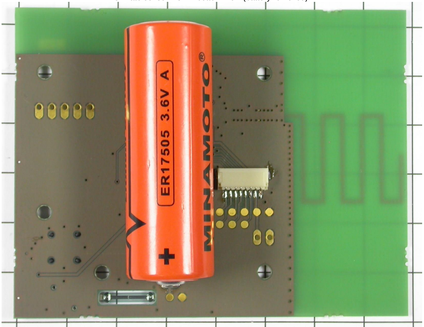
Climate sensor PCB – bottom view (battery removed)
