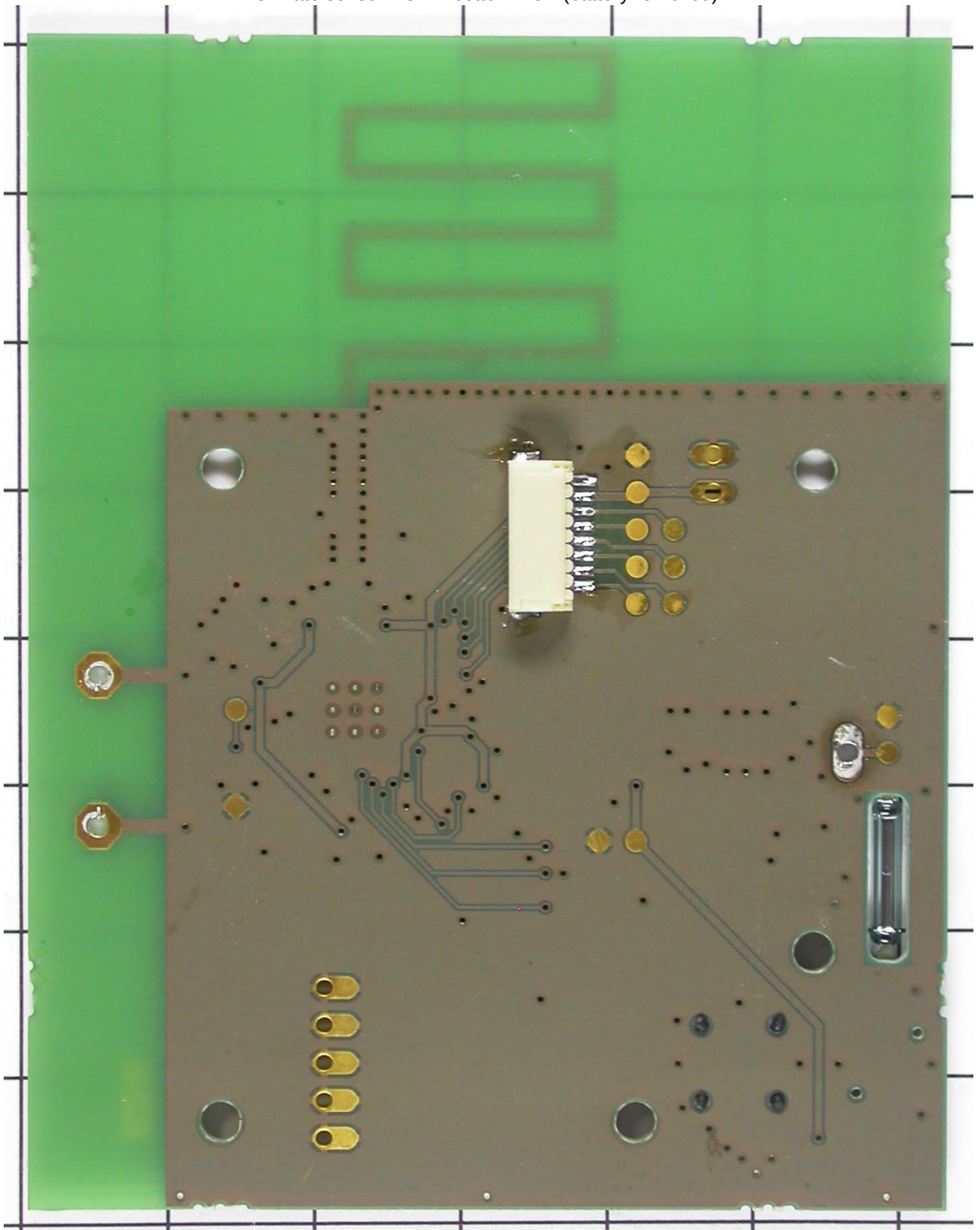
Climate sensor PCB – bottom view (battery removed)
