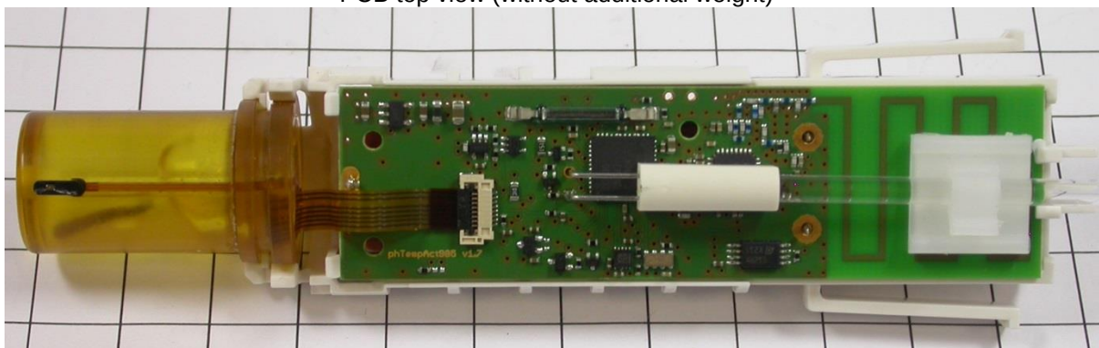
PCB top view (without additional weight)
