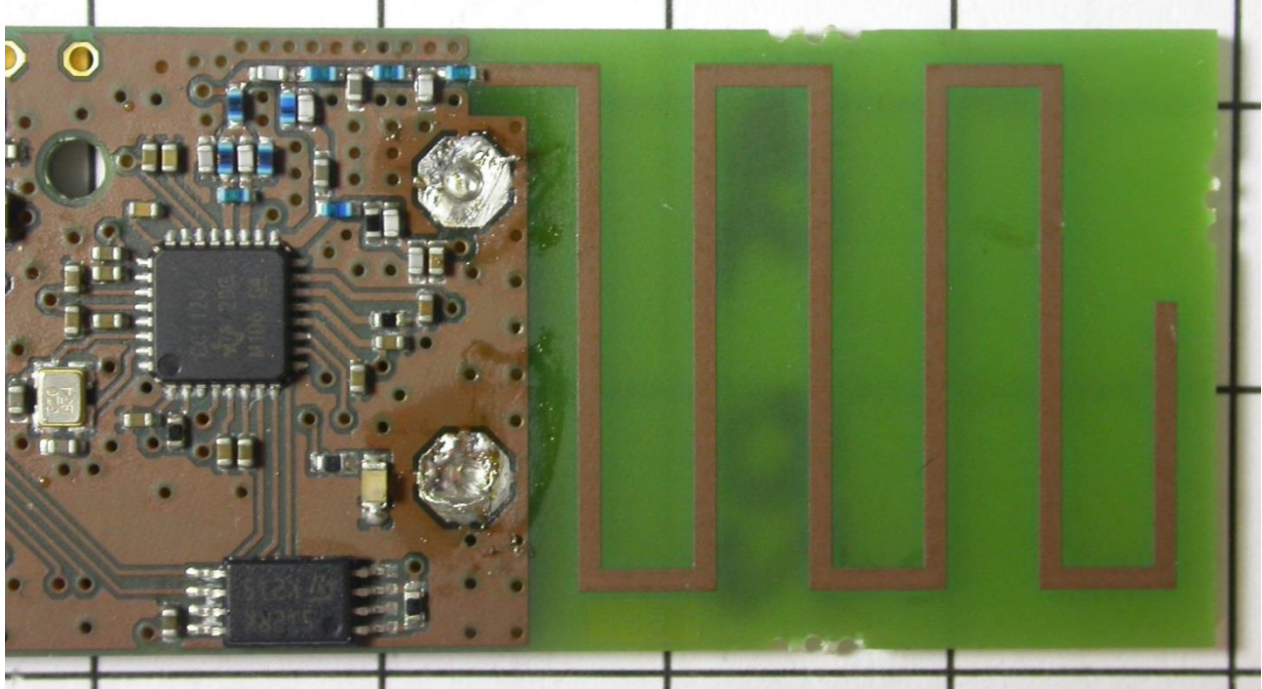
Printed antenna for 902 MHz to 928 MHz band – enlarged view
