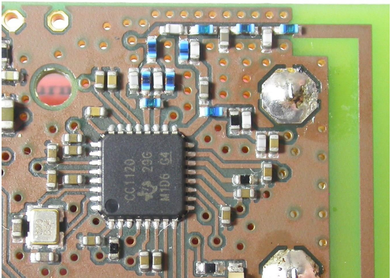
RF part for 902 MHz to 928 MHz band – enlarged view
