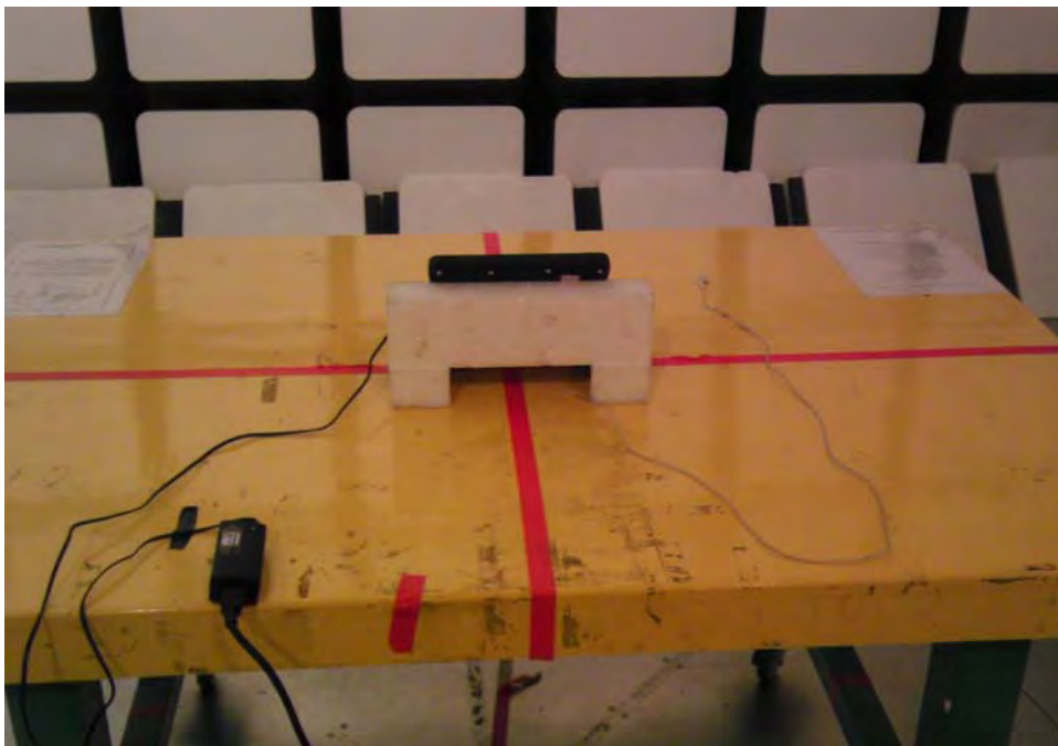
Below 1GHz _ Rear View_ Mode 3
