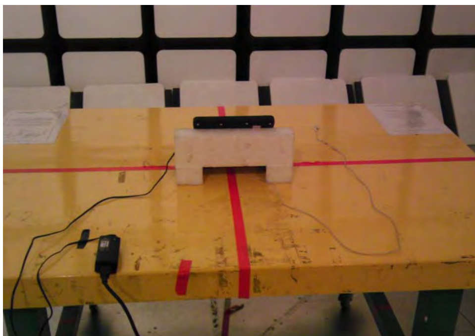
Above 1GHz _ Rear View_Mode 3
