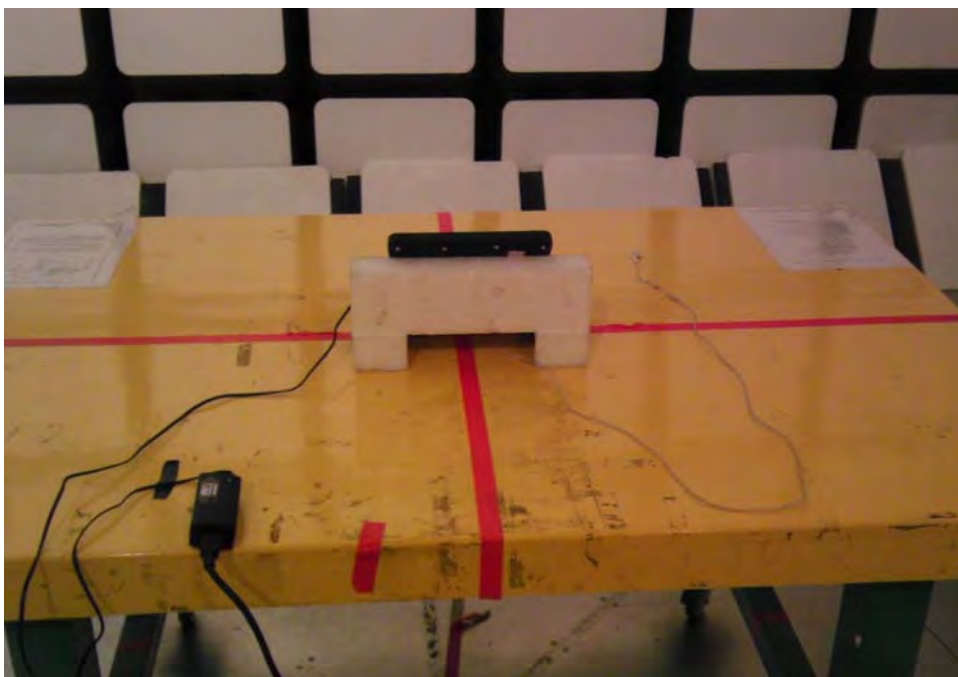
Below 1GHz _ Rear View _ Mode 3 / Mode 4
