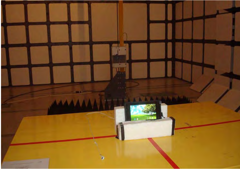
Above 1GHz _ Rear View _ Mode 1 / Mode 2
