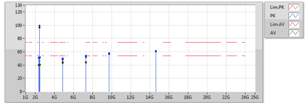
RE above 1GHz;Band:2.4G;11b;BWch:20MHz;Nss:1;Nant:1;Ch:2437MHz;TX
