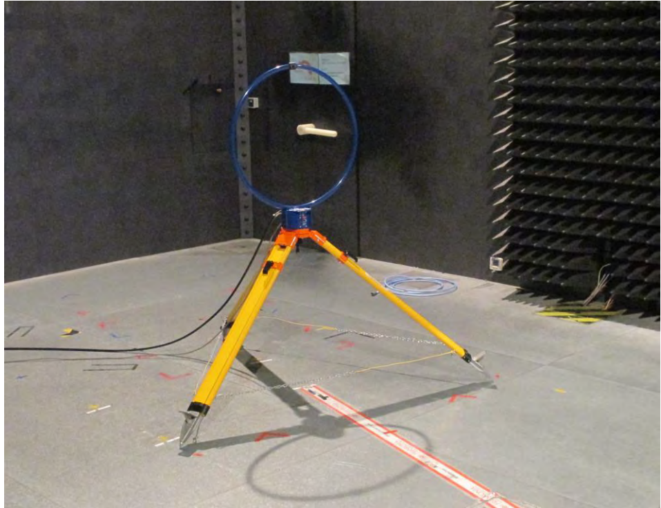
FRONT VIEW
