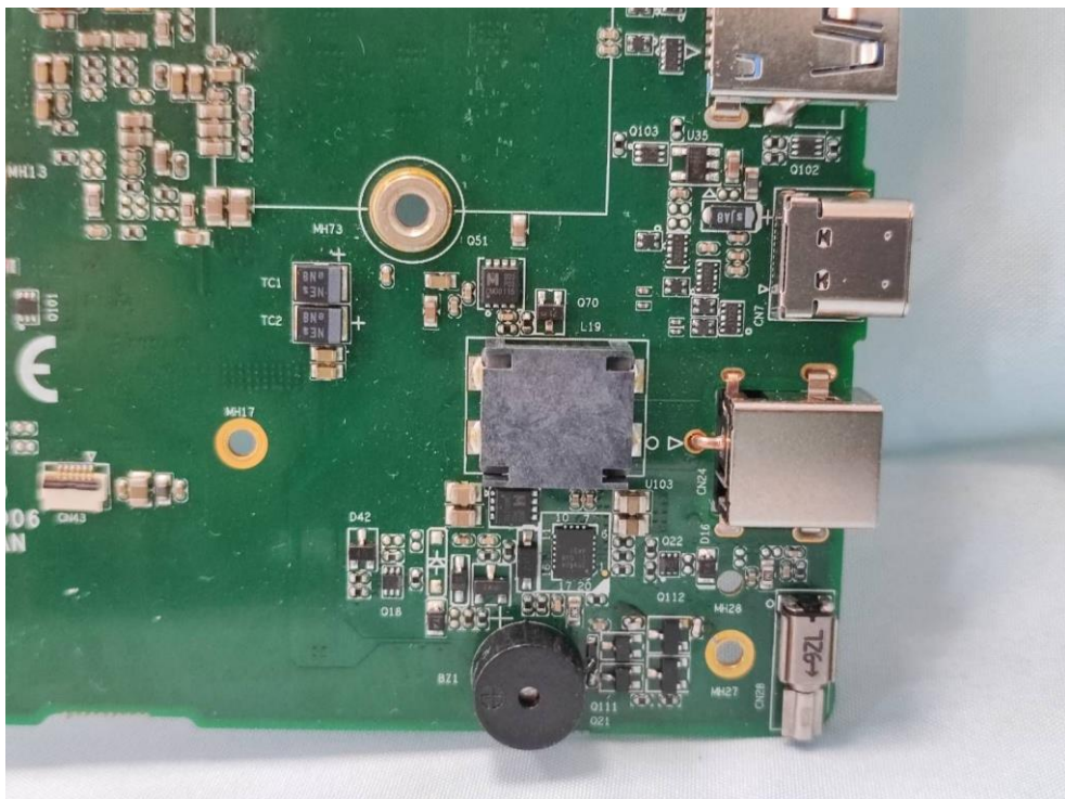
(28) EUT Photo
