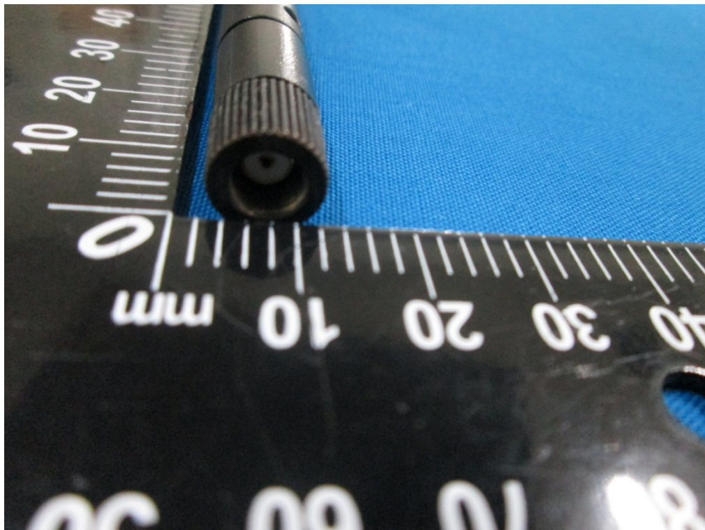
Dipole Antenna Port (Wi-Fi and Bluetooth)
