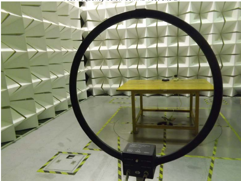
Test frequency below 30MHz Test Site 2#
