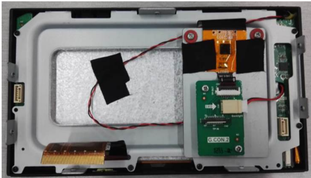
New panel (Model U621P, NV2400)
