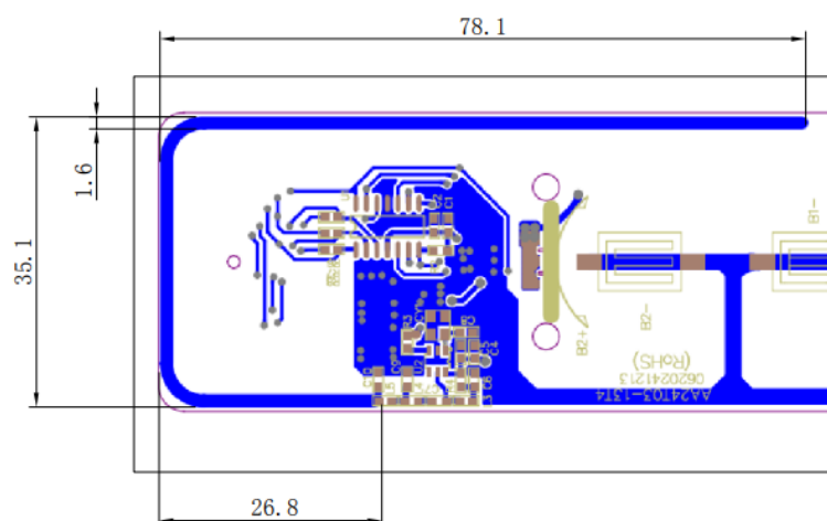
AA24T06-13T4 Schematic diagram of antenna position
