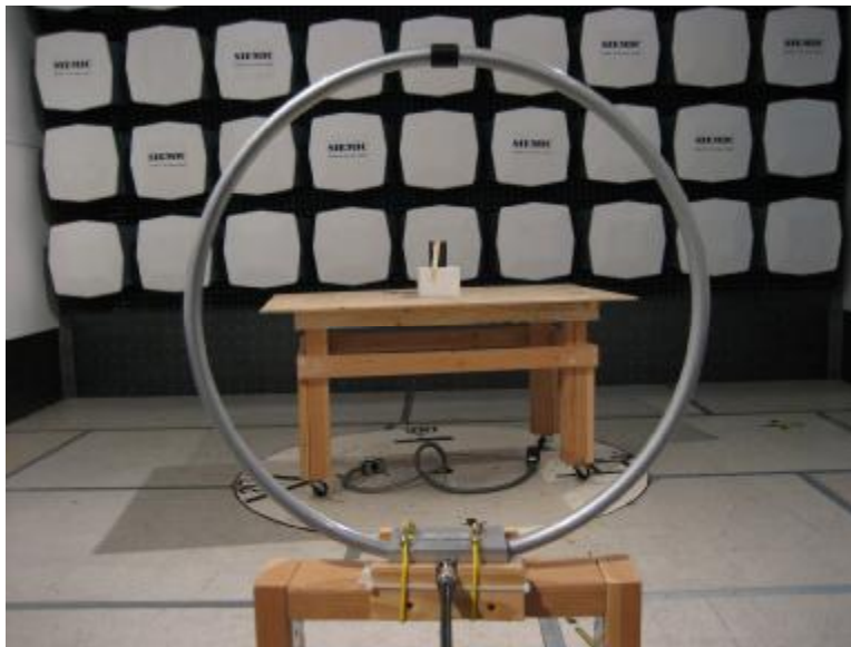
Radiated Emission setup < 30 MHz
