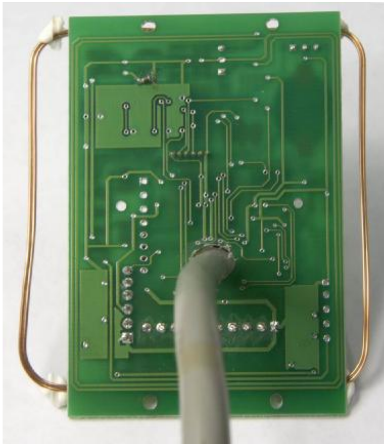
RF MAIN BOARD – BOTTOM SIDE
