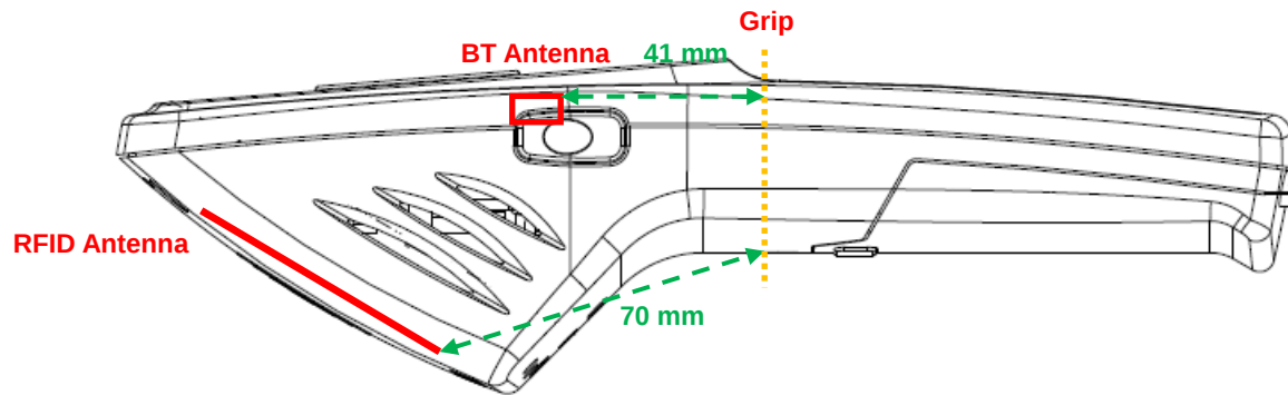
EUT Side View
