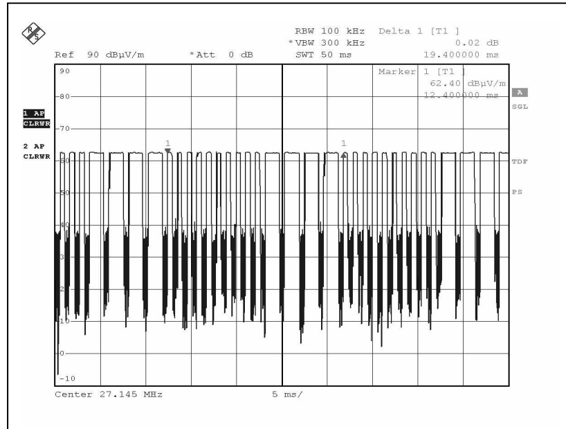
Duty Cycle 1
