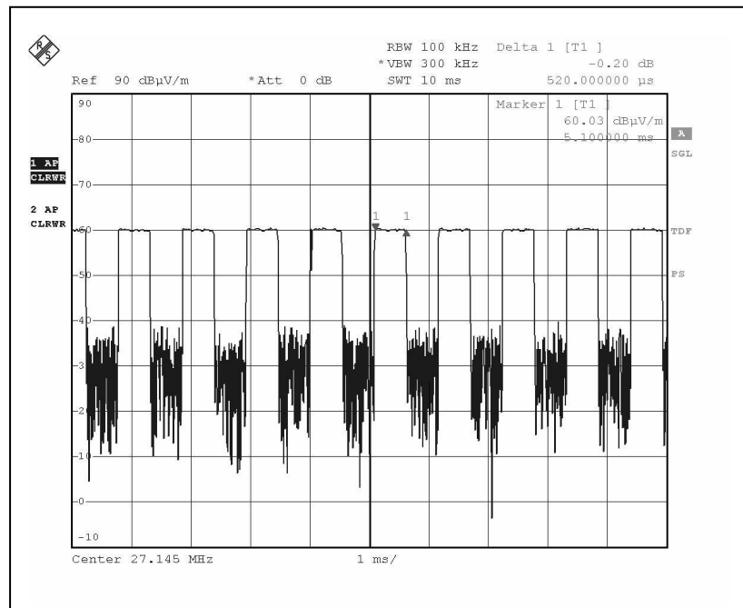
Duty Cycle 2
