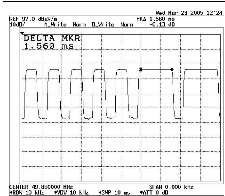
Duty Cycle 1
