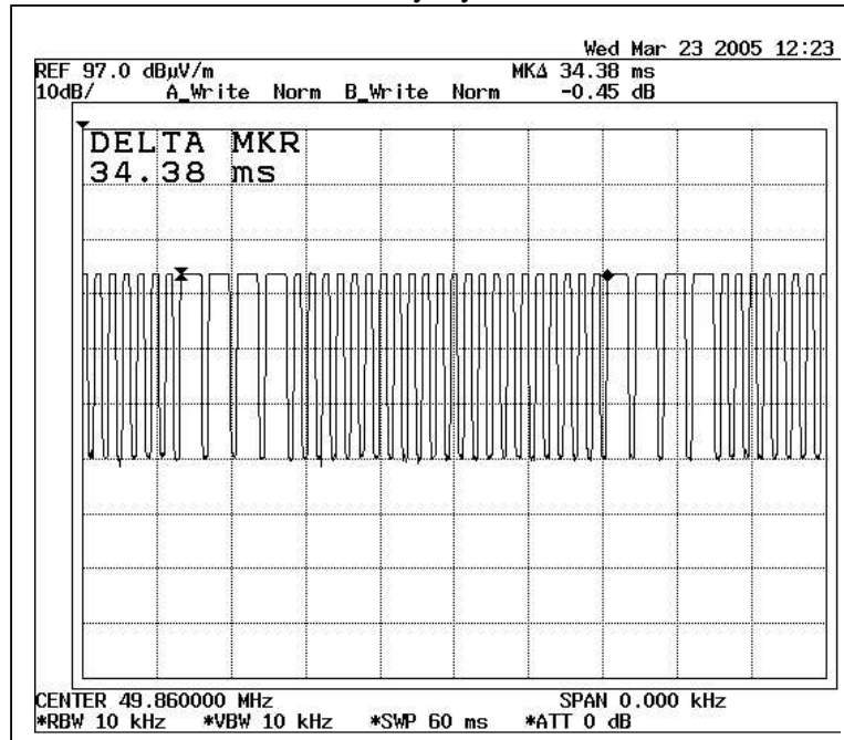
Duty Cycle
