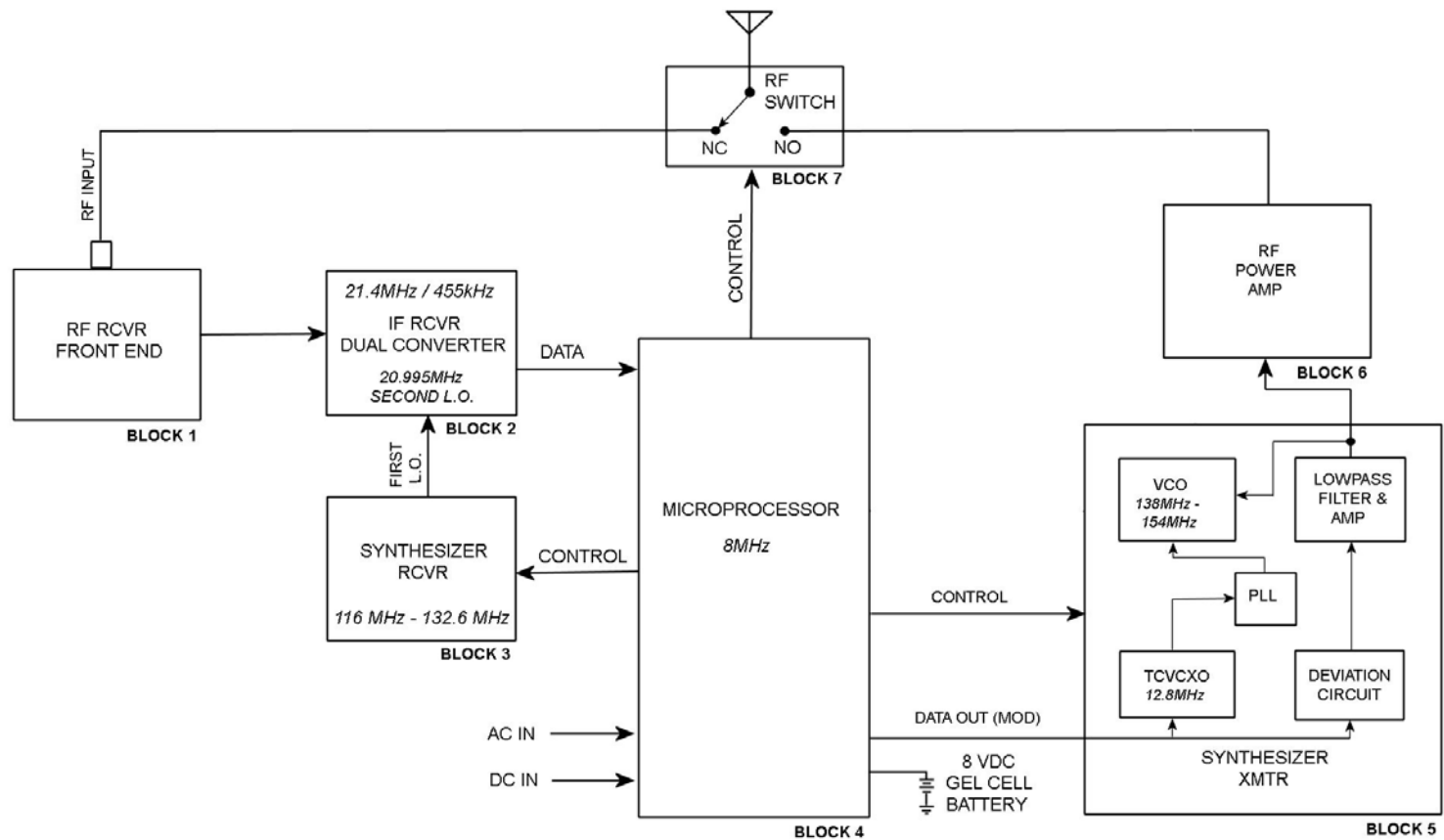
MRSY BLOCK DIAGRAM
