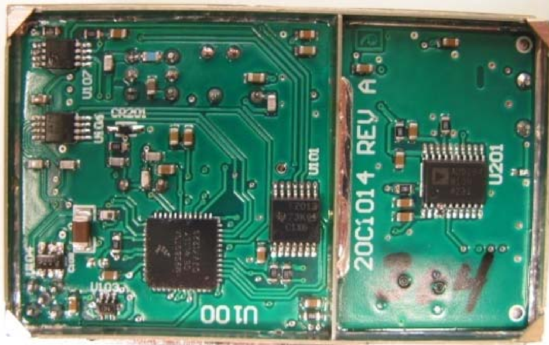
MCDR bottom pcb with shield
