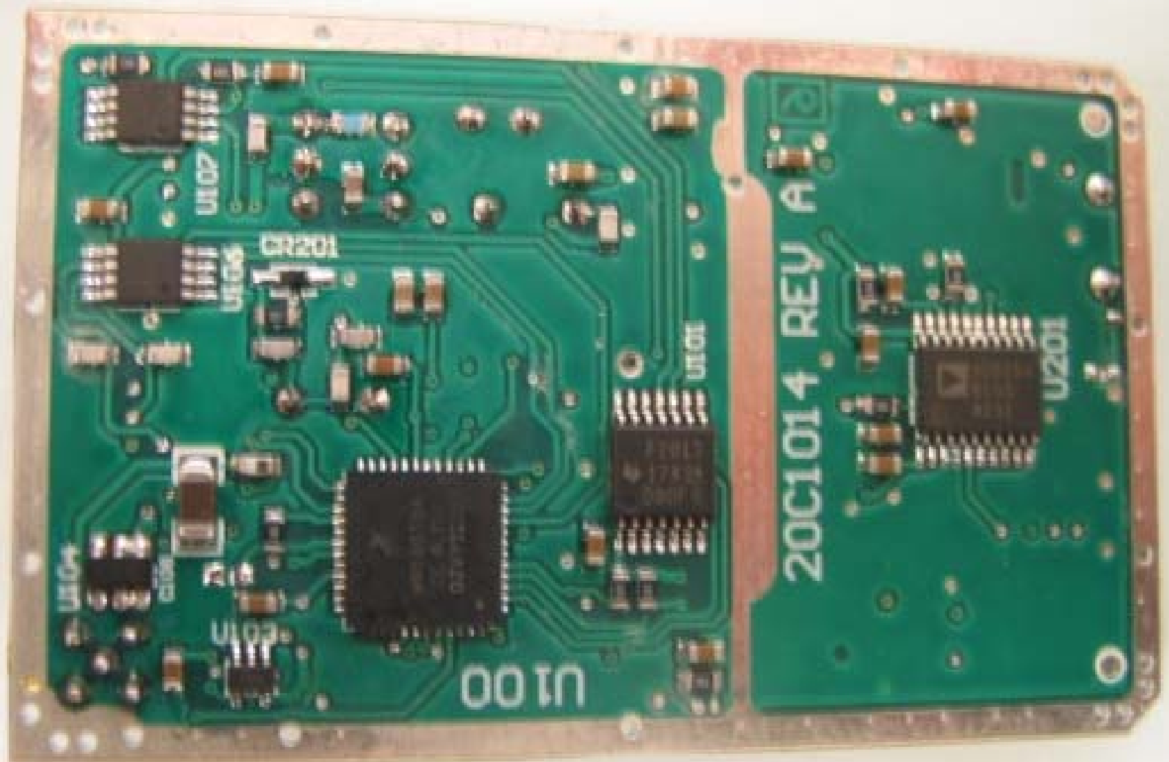
MCDR board bottom without shields
