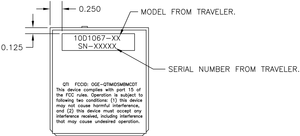
BOTTOM SHIELD OF MCDT MID BAND
