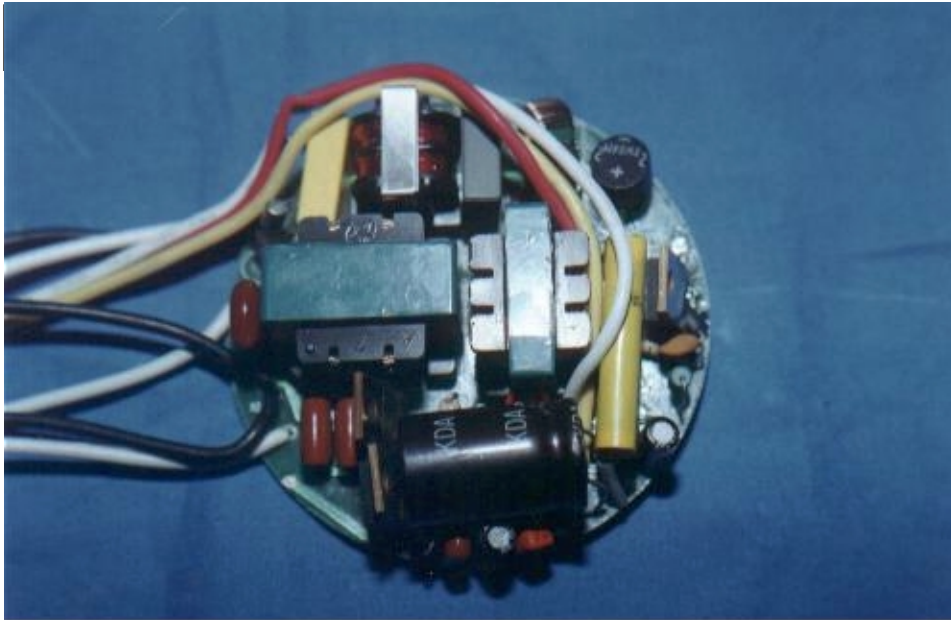
Main Board, Component Side
