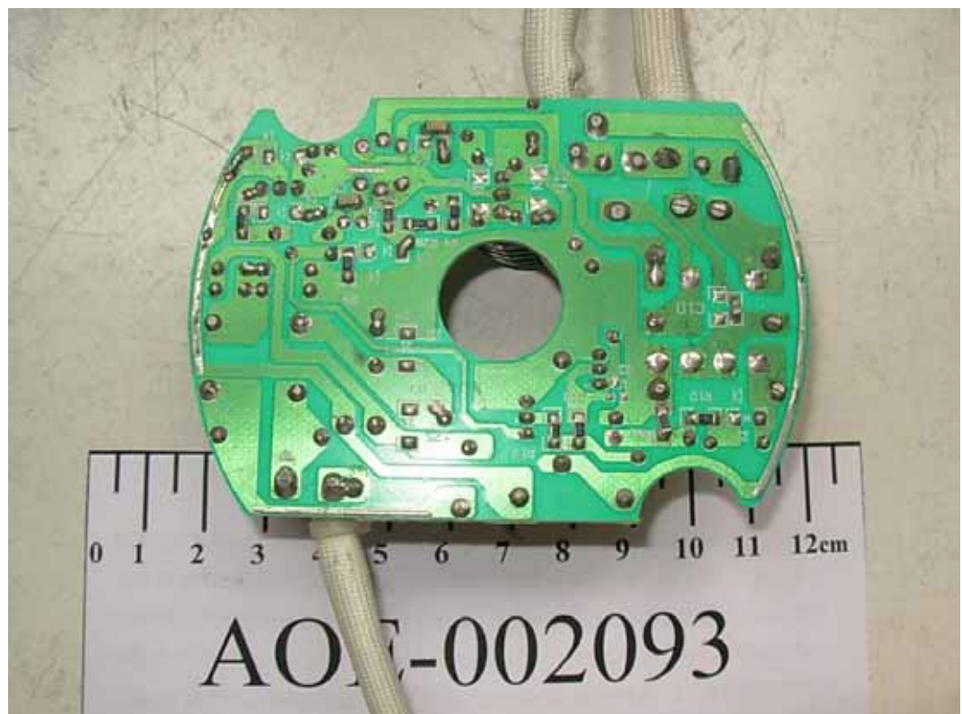
FIGURE 12 BALLAST (M/N: VEB82234) MAIN BOARD (SOLDERED SIDE)
