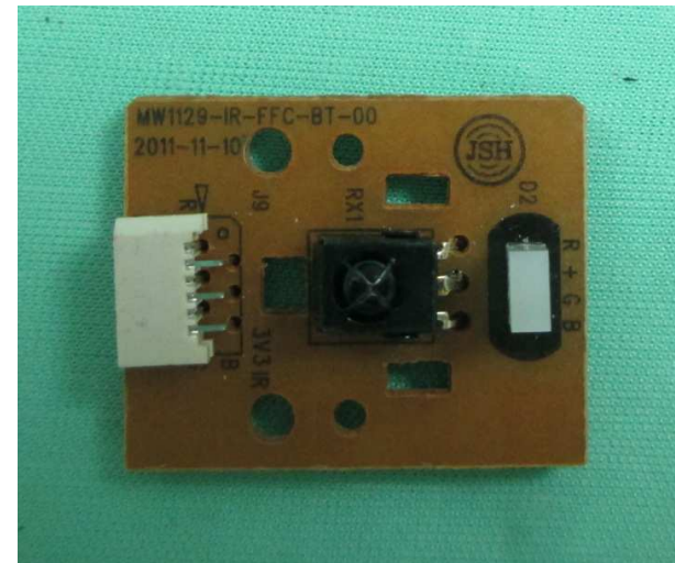
MODULE - INNER CIRCUIT TOP VIEW
