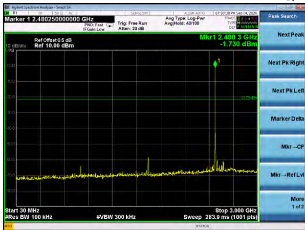
Pi/4 DQPSK High Channel
