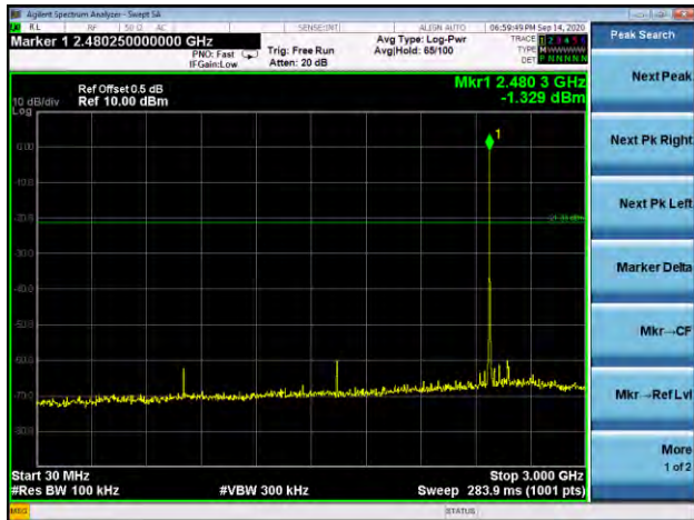
8DPSK High Channel
