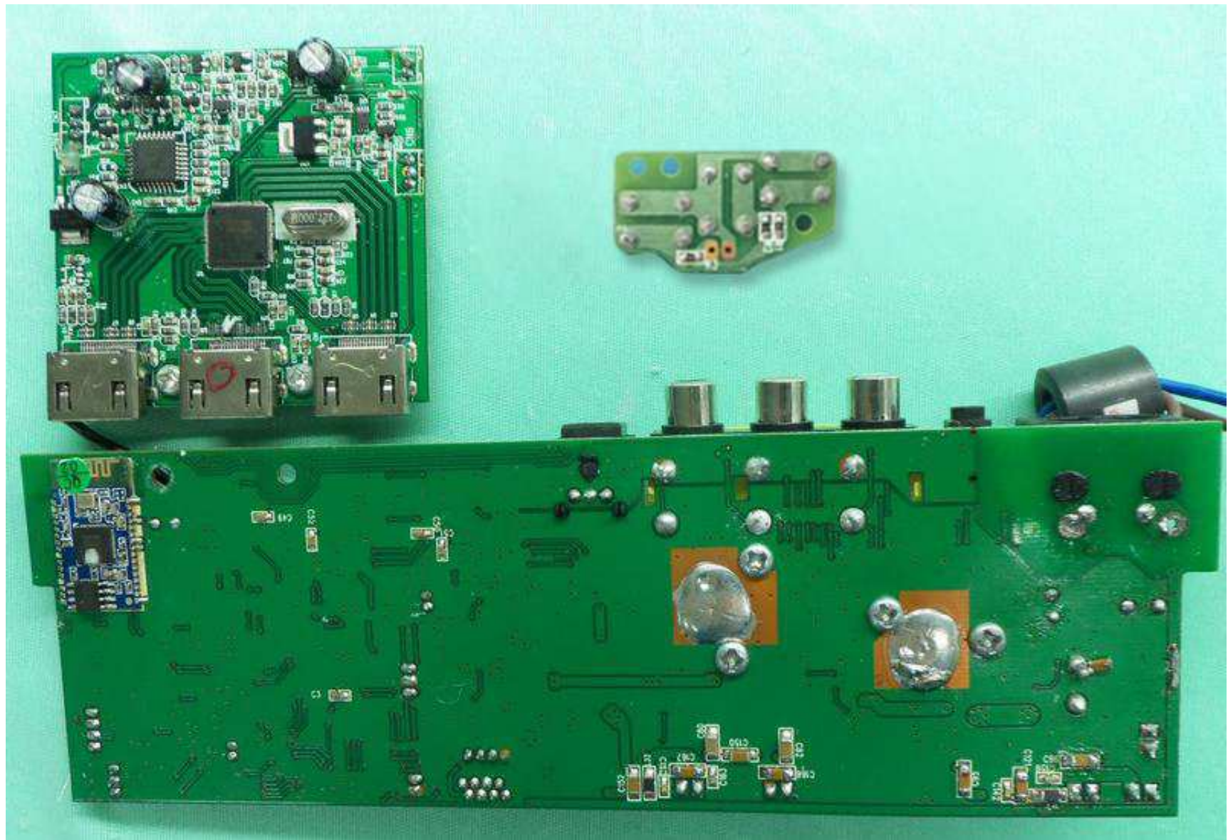
OG5MW-1587 PHOTOGRAPH OF THE PRODUCT INNER CIRCUIT BOTTOM VIEW
