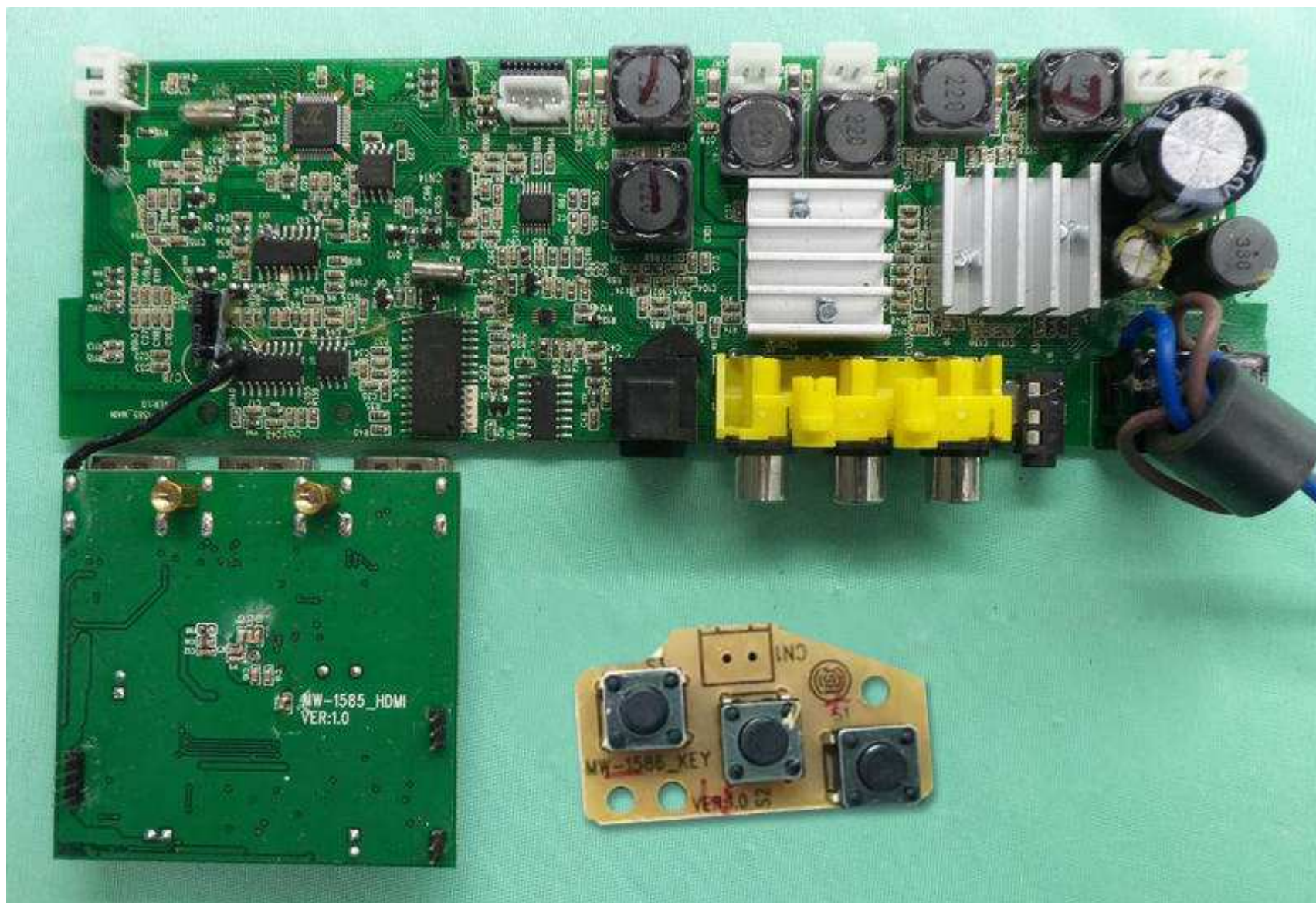
OG5MW-1587 PHOTOGRAPH OF THE PRODUCT INNER CIRCUIT TOP VIEW
