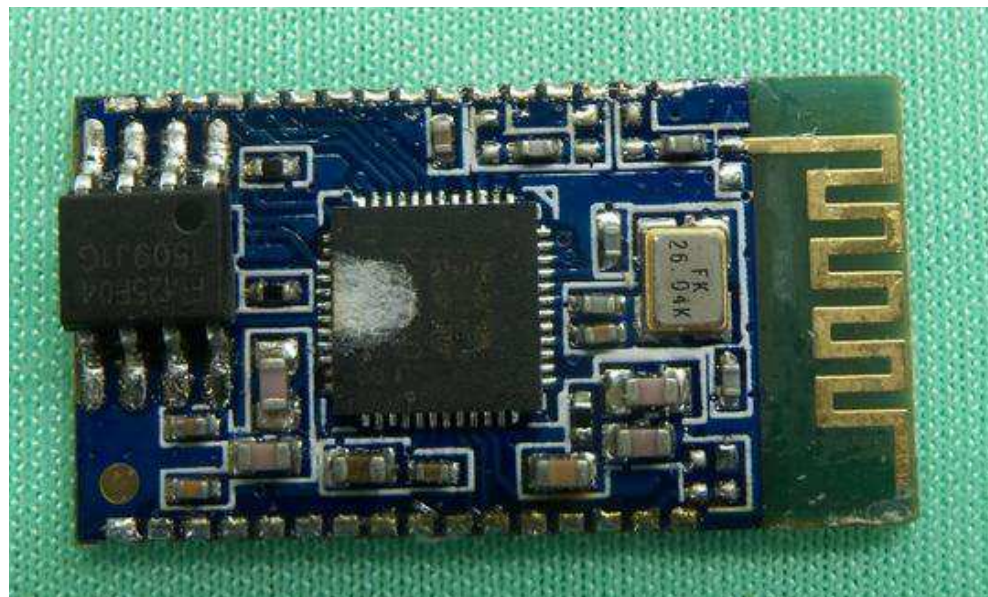
OG5MW-1587 PHOTOGRAPH OF THE PRODUCT
