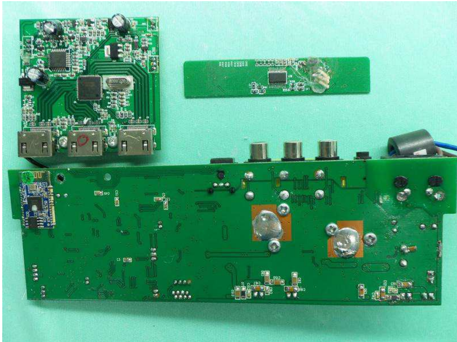
OG5MW-1585 PHOTOGRAPH OF THE PRODUCT INNER CIRCUIT BOTTOM VIEW
