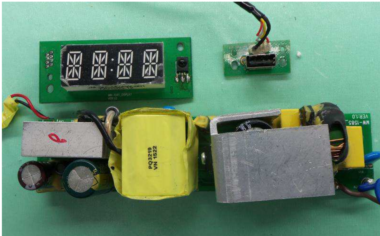
OG5MW-1585 PHOTOGRAPH OF THE PRODUCT
