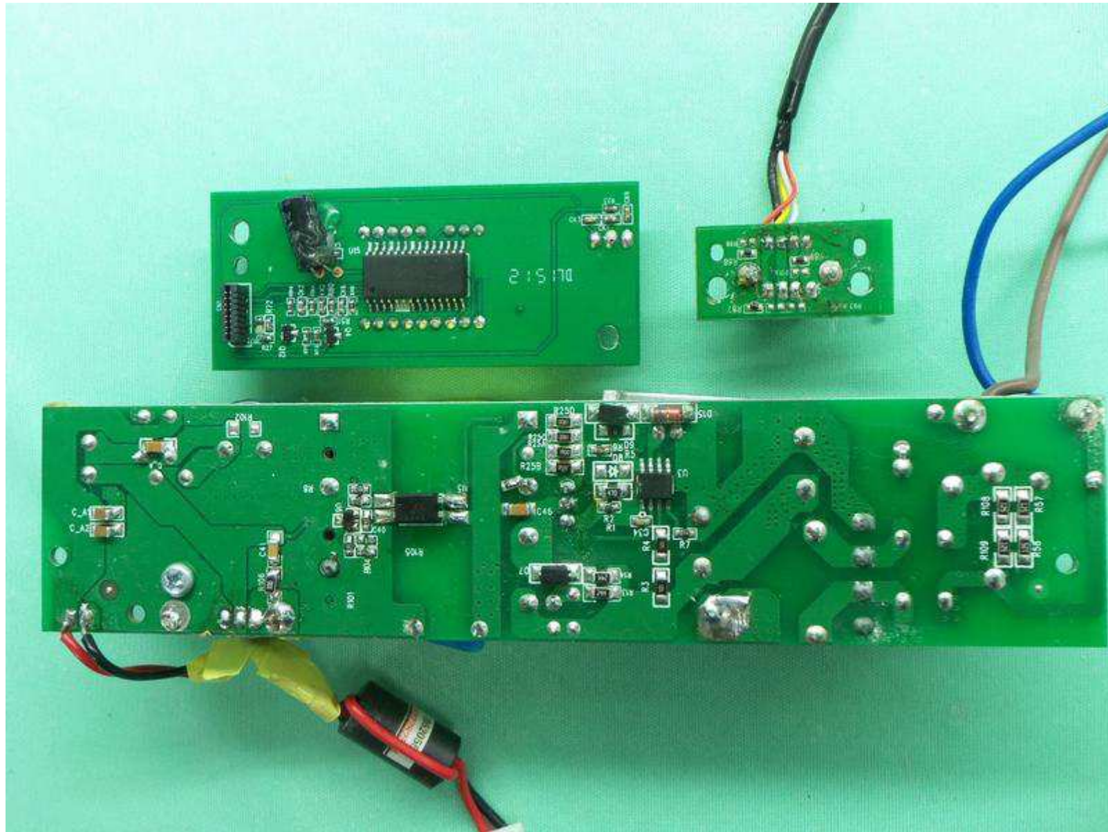
OG5MW-1585 PHOTOGRAPH OF THE PRODUCT
