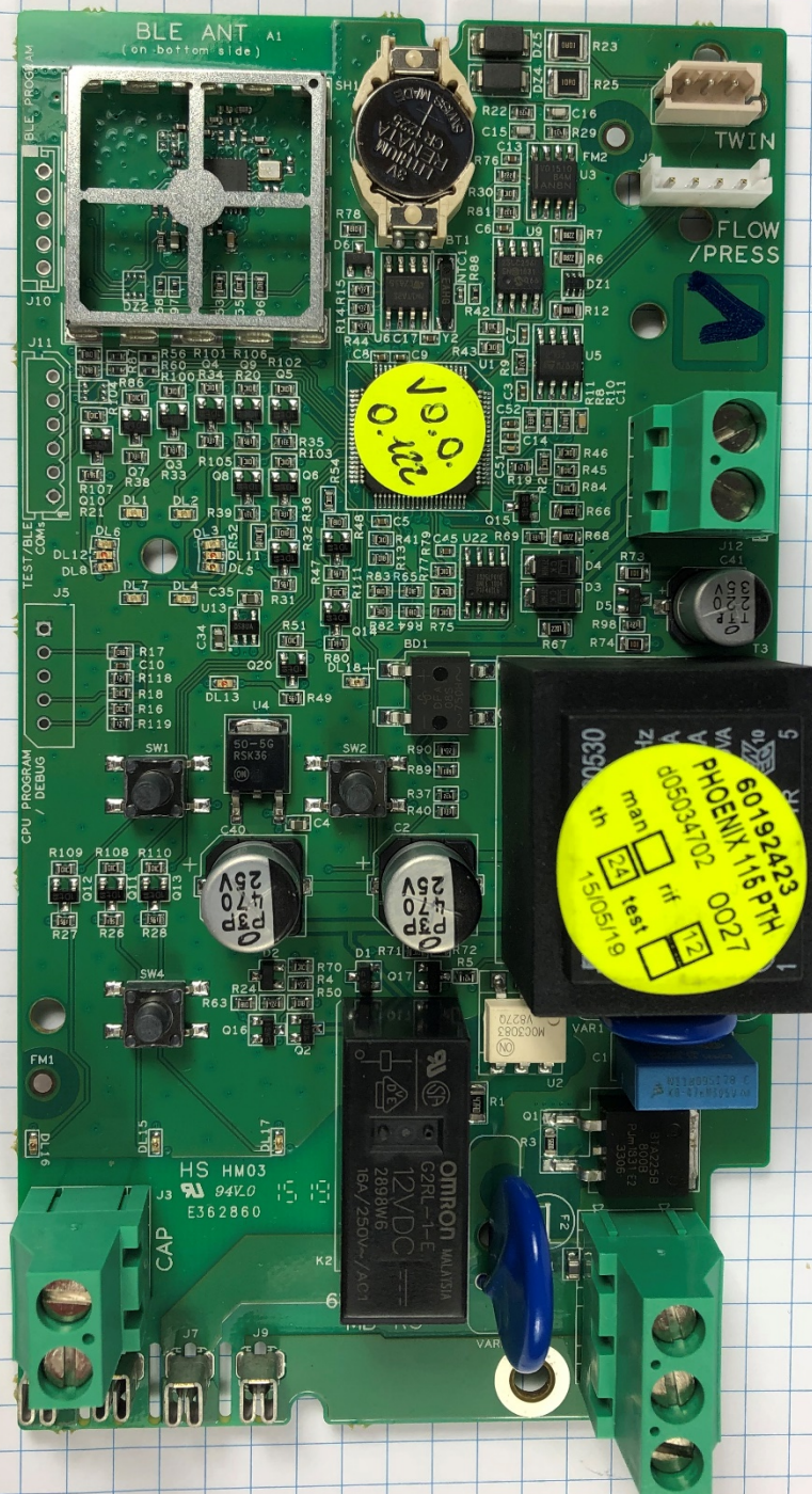
Figure 2 Top view "SCALA1" without RF shield
