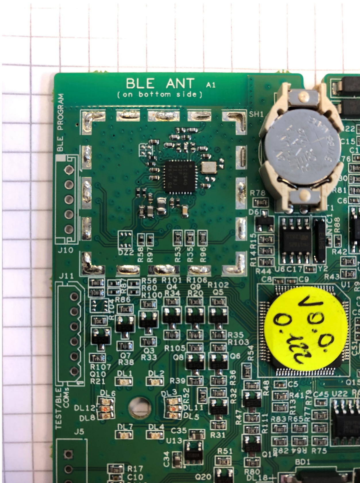
Figure 4 RF parts without screen frame
