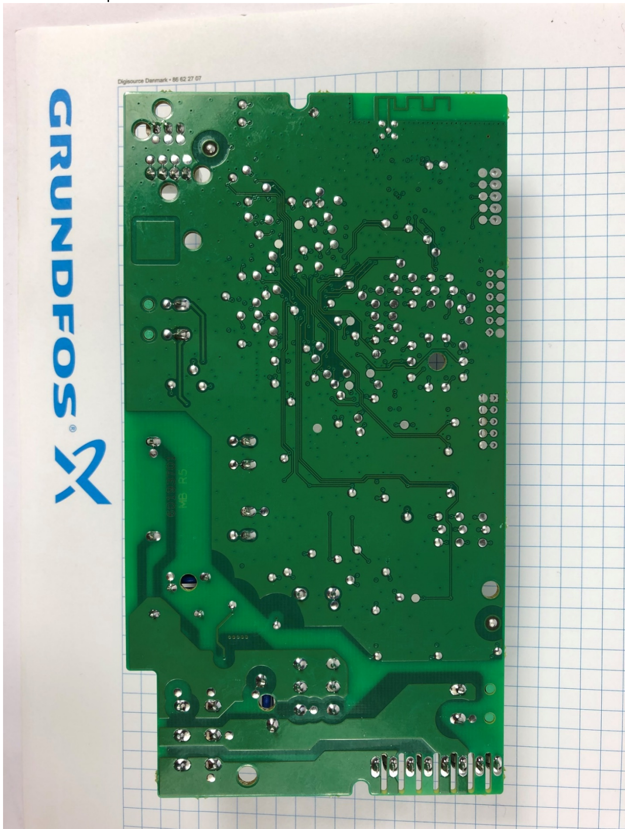
Figure 1 Bottom view of "SCALA1"
