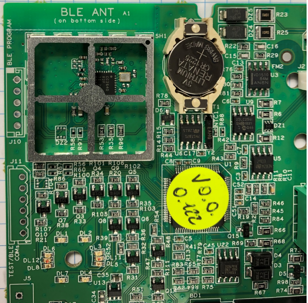
Figure 3 Closeup of RF parts under shield
