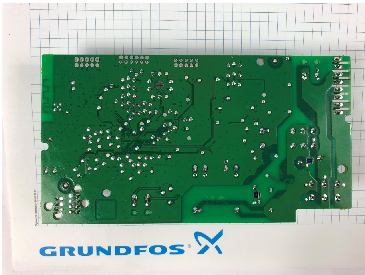
Figure 2 Radio module "OG3-SCALA1". Bottom side
