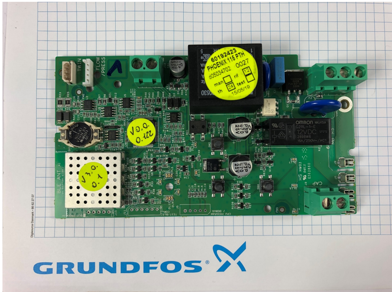
Figure 1 Radio module "OG3-SCALA1". Top side. RF parts under shield box
